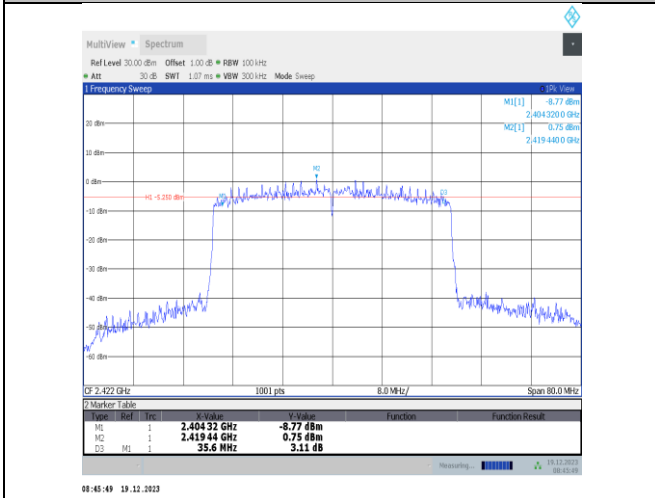
11ax40MIMO-Ant1-2422-PASS
