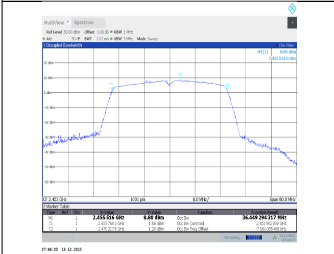
11n40SISO-Ant2-2452
