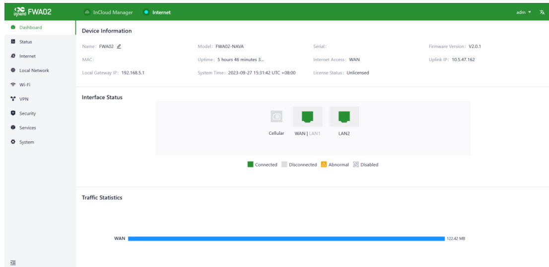
Fig. 5-1 Dashboard interface
