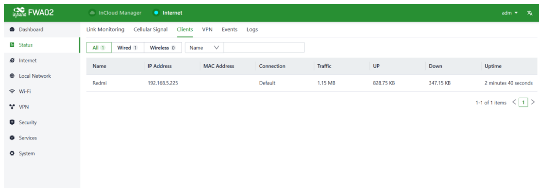
Fig. 5-2-3 Clients panel
