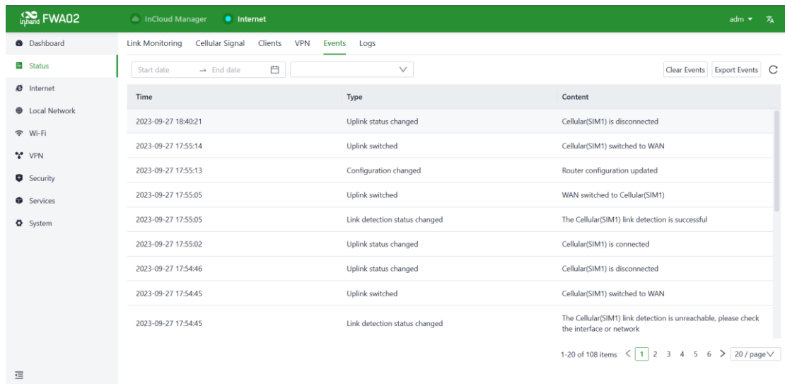
Fig. 5-2-5 Events interface
