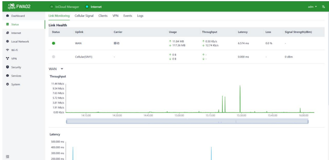
Fig. 5-2 Status interface
