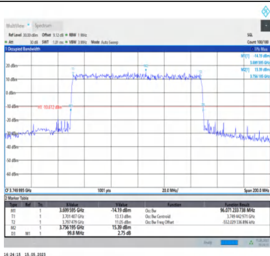
1-N77-3700-3980-PC1-30-100-L-1-DFT-QPSK-Outer_Full-270@0-Ant1-96.071-99.800-≤100-PASS
