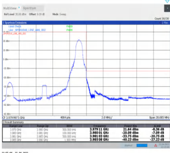
1-N77-3700-3980--30-10-H-5-CP-QPSK-Edge_1RB_R ight-1@23-Ant1-PASS-see graph
