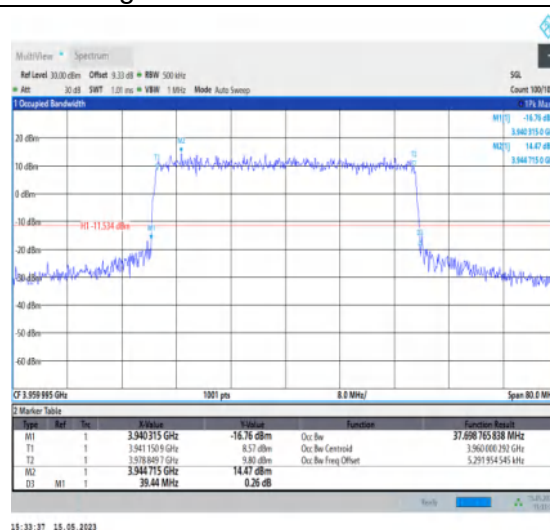
1-N77-3700-3980-PC1-30-40-H-8-CP-64QAM-Outer_Full-106@0-Ant1-37.699-39.440-≤40-PASS
