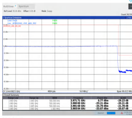
1-N77-3700-3980--30-80-H-6-CP-QPSK-Outer_Full-217@0-Ant1-PASS-see graph
