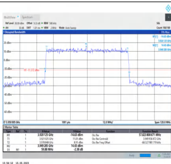
1-N77-3700-3980-PC1-30-60-H-1-DFT-QPSK-Out_ Full-162@0-Ant1-57.824-59.880-≤60-PASS
