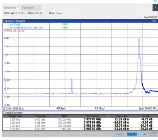
1-N77-3700-3980--30-80-H-5-CP-QPSK-Edge_1RB_Right-1@216-Ant1-PASS-see graph
