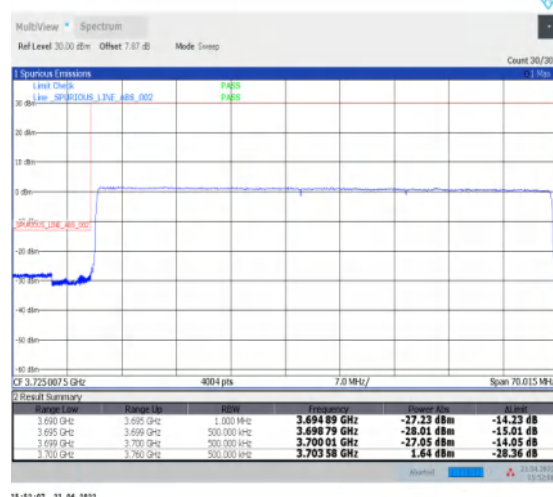
1-N77-3700-3980--30-60-L-6-CP-QPSK-Outer_Ful I-162@0-Ant1-PASS-see graph
