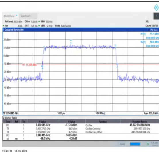
1-N77-3700-3980-PC1-30-50-H-4-DFT-64QAM-Outer_Full-128@0-Ant1-45.522-48.000-≤50-PASS
