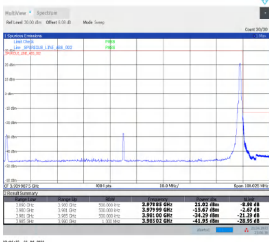
1-N77-3700-3980--30-90-H-5-CP-QPSK-Edge_1RB_R ight-1@244-Ant1-PASS-see graph
