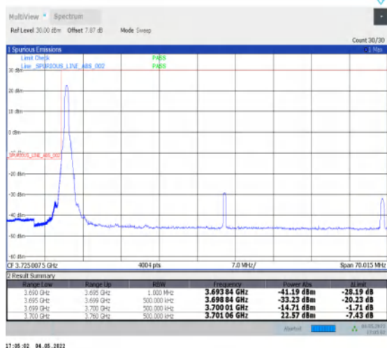
1-N77-3700-3980--30-60-L-1-DFT-PI2BPSK-Edge_1R_B_Left-1@0-Ant1-PASS-see graph
