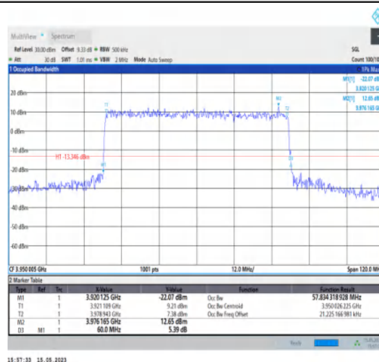
1-N77-3700-3980-PC1-30-60-H-8-CP-64QAM-Outer_Full-162@0-Ant1-57.834-60.000-≤60-PASS
