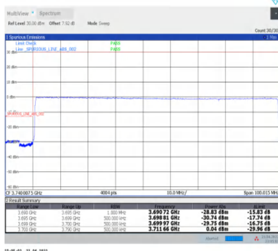
1-N77-3700-3980--30-90-L-6-CP-QPSK-Outer_Ful I-245@0-Ant1-PASS-see graph
