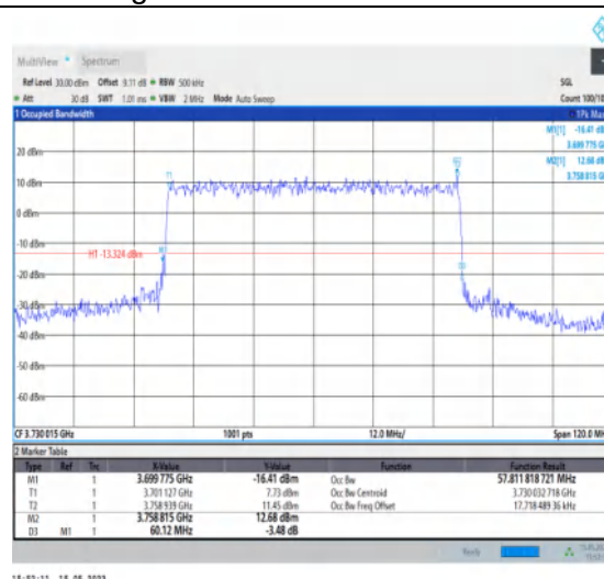
1-N77-3700-3980-PC1-30-60-L-8-CP-64QAM-Outer_Full-162@0-Ant1-57.812-60.120-≤60-PASS
