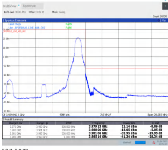
1-N77-3700-3980--30-10-H-2-DFT-PI2BPSK-Edge_1R_B_Right-1@23-Ant1-PASS-see graph
