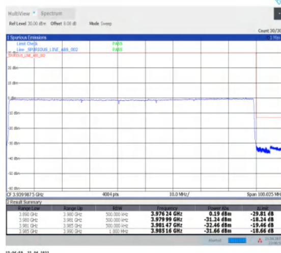
1-N77-3700-3980--30-90-H-6-CP-QPSK-Outer_Fu ll-245@0-Ant1-PASS-see graph
