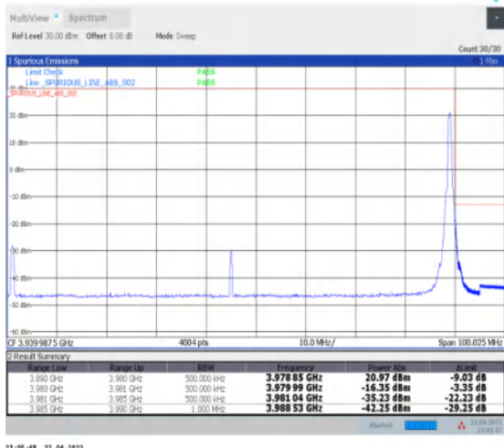
1-N77-3700-3980--30-90-H-2-DFT-PI2BPSK-Edge_1R_B_Right-1@244-Ant1-PASS-see graph
