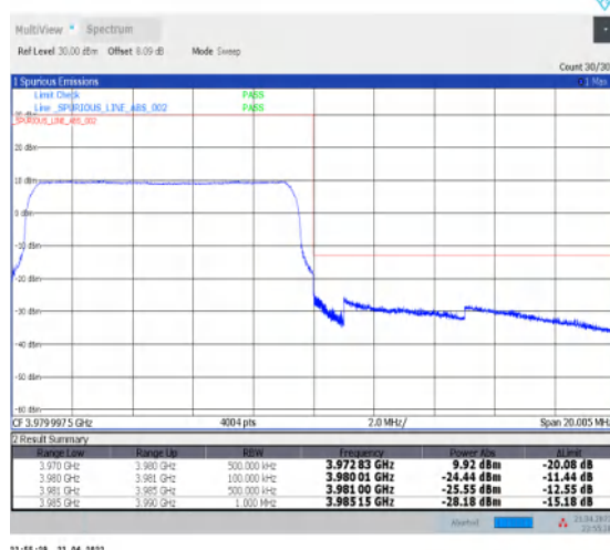
1-N77-3700-3980--30-10-H-6-CP-QPSK-Outer_Fu ll-24@0-Ant1-PASS-see graph
