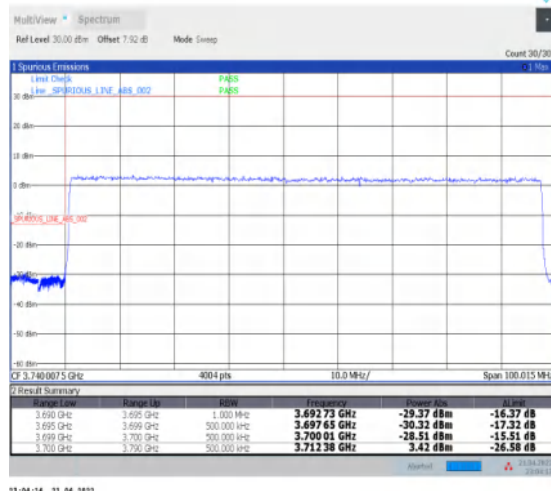
1-N77-3700-3980--30-90-L-3-DFT-PI2BPSK-Outer_Full-240@0-Ant1-PASS-see graph
