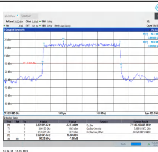
1-N77-3700-3980-PC1-30-80-H-2-DFT-PI2BPSK-Outer_Full-216@0-Ant1-77.189-80.320-≤80-PASS
