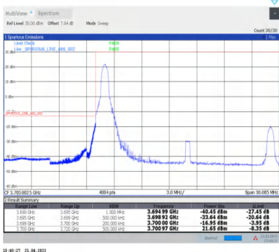
1-N77-3700-3980--30-20-L-4-CP-QPSK-Edge_1RB_L eft-1@0-Ant1-PASS-see graph
