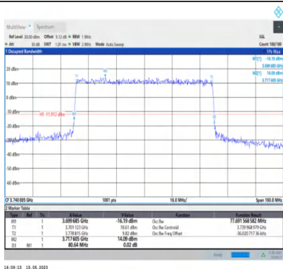
1-N77-3700-3980-PC1-30-80-L-7-CP-16QAM-Outer_Full-217@0-Ant1-77.692-80.640-≤80-PASS
