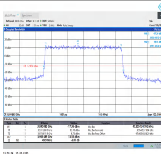
1-N77-3700-3980-PC1-30-50-H-7-CP-16QAM-Outer_Full-133@0-Ant1-47.356-49.900-≤50-PASS
