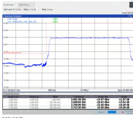
1-N77-3700-3980--30-20-L-3-DFT-PI2BPSK-Outer_Full-50@0-Ant1-PASS-see graph
