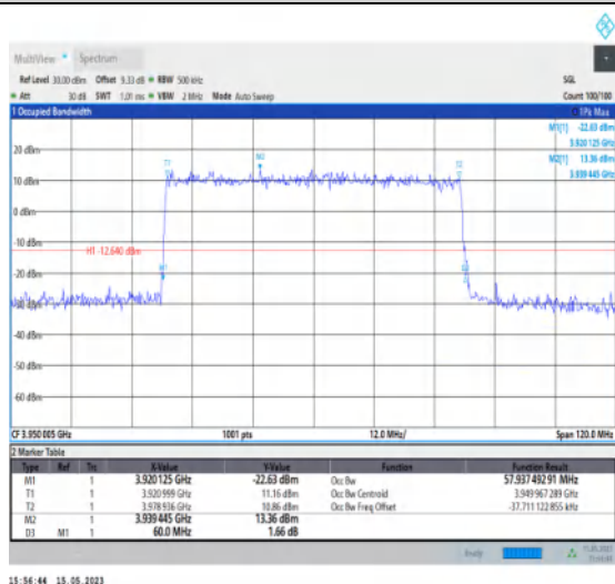
1-N77-3700-3980-PC1-30-60-H-3-DFT-16QAM-Oute r_Full-162@0-Ant1-57.937-60.000-≤60-PASS
