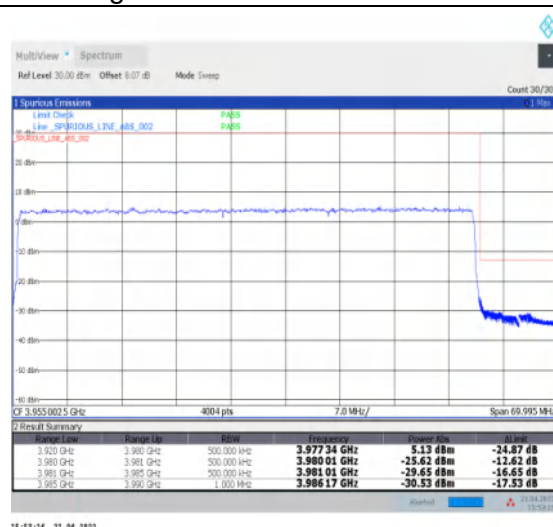
1-N77-3700-3980--30-60-H-3-DFT-PI2BPSK-Outer_Full-162@0-Ant1-PASS-see graph
