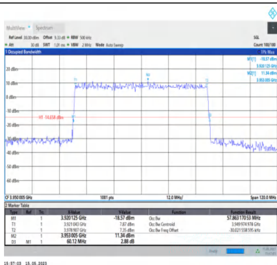
1-N77-3700-3980-PC1-30-60-H-5-DFT-256QAM-Out_er_Full-162@0-Ant1-57.863-60.120-≤60-PASS
