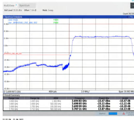
1-N77-3700-3980--30-10-L-3-DFT-PI2BPSK-Outer _Full-24@0-Ant1-PASS-see graph
