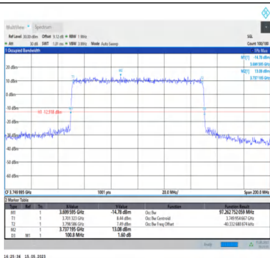
1-N77-3700-3980-PC1-30-100-L-7-CP-16QAM-Outer_Full-273@0-Ant1-97.263-100.800-≤100-PASS
