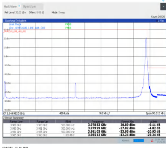
1-N77-3700-3980--30-80-H-2-DFT-PI2BPSK-Edge_1R_B_Right-1@216-Ant1-PASS-see graph
