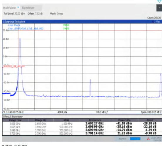
1-N77-3700-3980--30-90-L-4-CP-QPSK-Edge_1RB_L eft-1@0-Ant1-PASS-see graph
