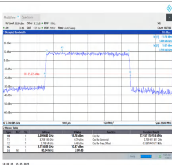
1-N77-3700-3980-PC1-30-80-L-9-CP-256QAM-Outer_Full-217@0-Ant1-77.457-80.640-≤80-PASS
