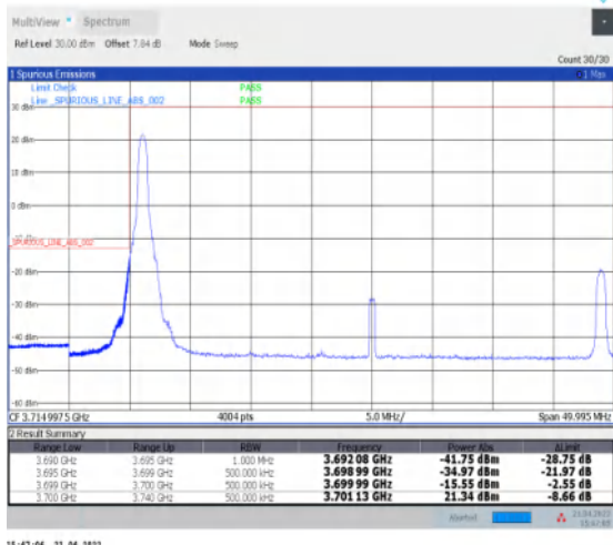
1-N77-3700-3980--30-40-L-1-DFT-PI2BPSK-Edge_1R_B_Left-1@0-Ant1-PASS-see graph
