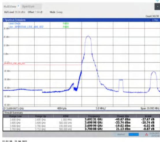
1-N77-3700-3980--30-10-L-1-DFT-PI2BPSK-Edge_1R B_Left-1@0-Ant1-PASS-see graph
