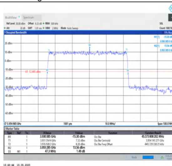
1-N77-3700-3980-PC1-30-50-H-5-DFT-256QAM-Outer_Full-128@0-Ant1-45.574-47.300-≤50-PASS
