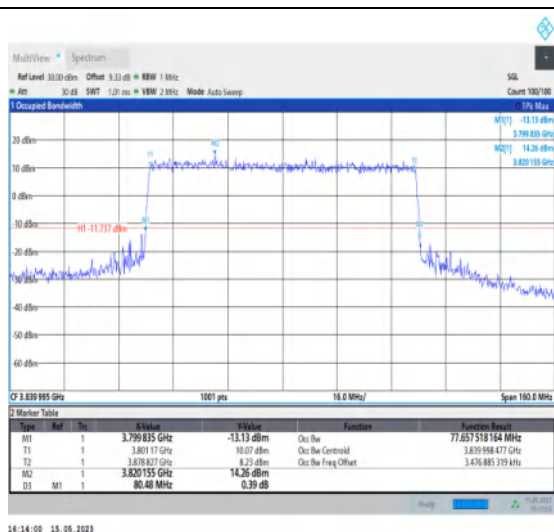
1-N77-3700-3980-PC1-30-80-M-8-CP-64QAM-Outer_Full-217@0-Ant1-77.658-80.480-≤80-PASS
