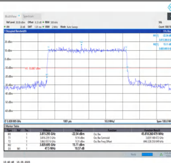
1-N77-3700-3980-PC1-30-50-M-4-DFT-64QAM-Outer_Full-128@0-Ant1-45.818-47.500-≤50-PASS
