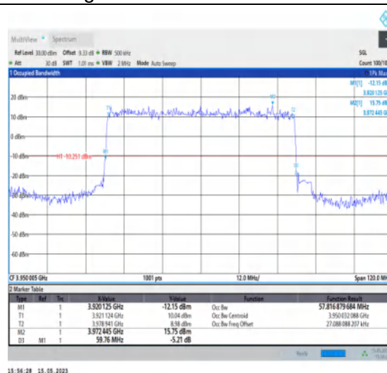
1-N77-3700-3980-PC1-30-60-H-2-DFT-PI2BPSK-Ou ter_Full-162@0-Ant1-57.817-59.760-≤60-PASS
