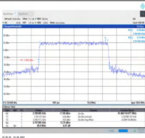
1-N77-3700-3980-PC1-30-50-L-8-CP-64QAM-Outer_Full-133@0-Ant1-47.46-49.400-≤50-PASS
