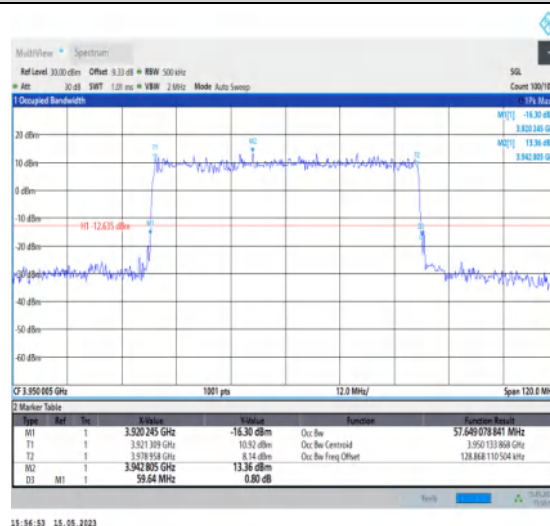
1-N77-3700-3980-PC1-30-60-H-4-DFT-64QAM-Out er_Full-162@0-Ant1-57.649-59.640-≤60-PASS
