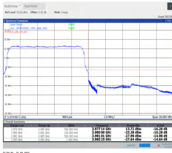
1-N77-3700-3980--30-10-H-3-DFT-PI2BPSK-Outer_Full-24@0-Ant1-PASS-see graph
