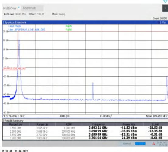
1-N77-3700-3980--30-100-L-4-CP-QPSK-Edge_1RB_ Left-1@0-Ant1-PASS-see graph
