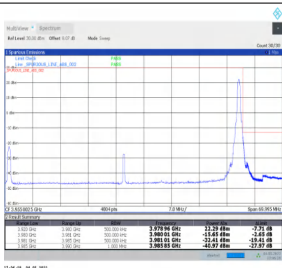
1-N77-3700-3980--30-60-H-2-DFT-PI2BPSK-Edge_1R_B_Right-1@161-Ant1-PASS-see graph
