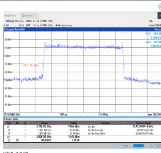
1-N77-3700-3980-PC1-30-80-M-7-CP-16QAM-Outer_Full-217@0-Ant1-77.412-80.800-≤80-PASS
