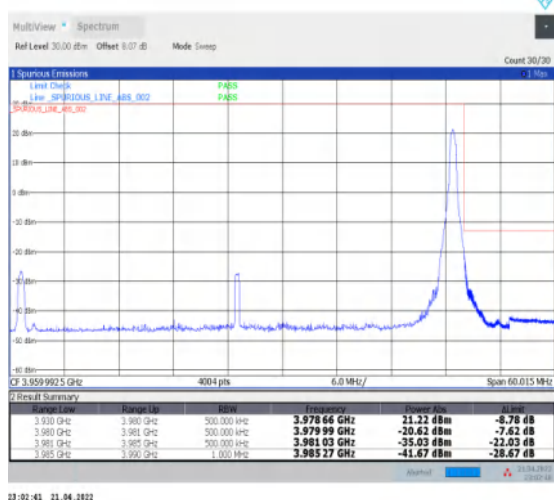
1-N77-3700-3980--30-50-H-5-CP-QPSK-Edge_1RB_Right-1@132-Ant1-PASS-see graph
