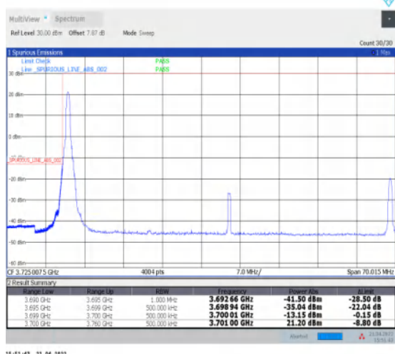
1-N77-3700-3980--30-60-L-4-CP-QPSK-Edge_1RB_L eft-1@0-Ant1-PASS-see graph
