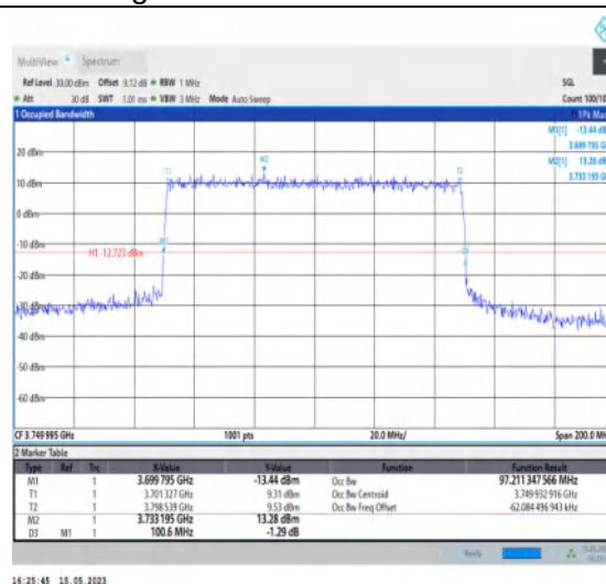
1-N77-3700-3980-PC1-30-100-L-8-CP-64QAM-Outer_Full-273@0-Ant1-97.211-100.600-≤100-PASS
