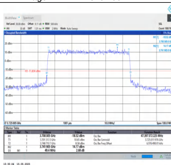
1-N77-3700-3980-PC1-30-50-L-7-CP-16QAM-Outer_Full-133@0-Ant1-47.397-49.400-≤50-PASS
