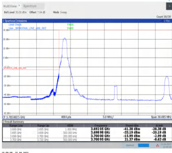
1-N77-3700-3980--30-20-L-1-DFT-PI2BPSK-Edge_1R_B_Left-1@0-Ant1-PASS-see graph
