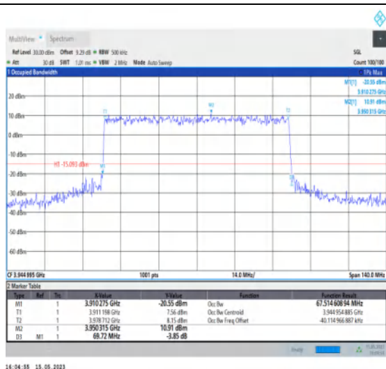
1-N77-3700-3980-PC1-30-70-H-6-CP-QPSK-Outer_Full-189@0-Ant1-67.515-69.720-≤70-PASS
