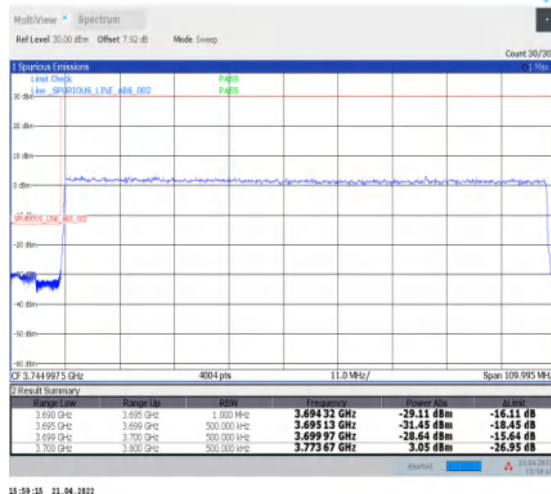
1-N77-3700-3980--30-100-L-3-DFT-PI2BPSK-Out er_Full-270@0-Ant1-PASS-see graph
