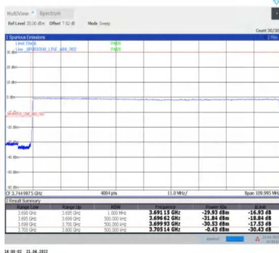
1-N77-3700-3980--30-100-L-6-CP-QPSK-Outer_F ull-273@0-Ant1-PASS-see graph
