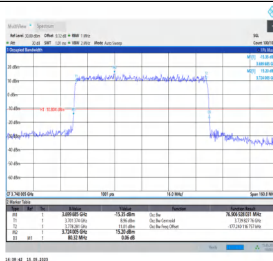
1-N77-3700-3980-PC1-30-80-L-4-DFT-64QAM-Outer_Full-216@0-Ant1-76.907-80.320-≤80-PASS
