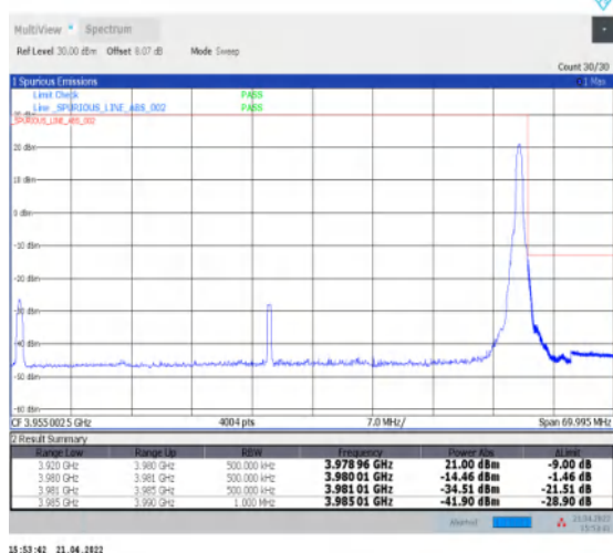
1-N77-3700-3980--30-60-H-5-CP-QPSK-Edge_1RB_Right-1@161-Ant1-PASS-see graph
