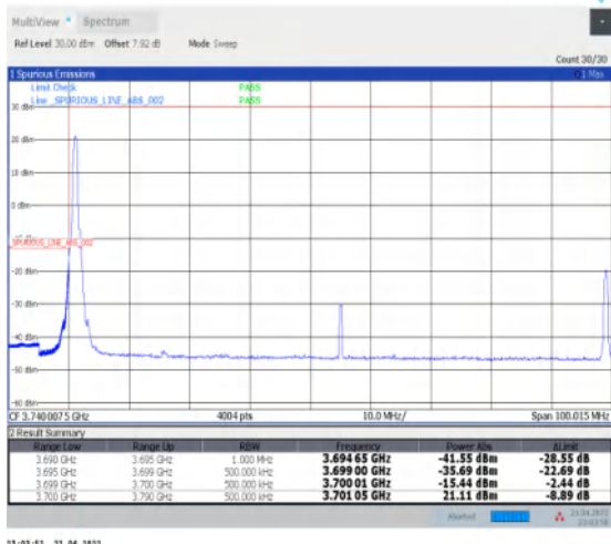
1-N77-3700-3980--30-90-L-1-DFT-PI2BPSK-Edge_1R_B_Left-1@0-Ant1-PASS-see graph
