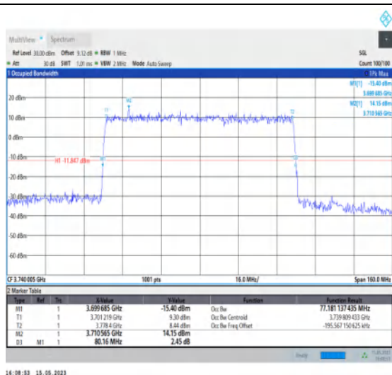
1-N77-3700-3980-PC1-30-80-L-5-DFT-256QAM-Out er_Full-216@0-Ant1-77.181-80.160-≤80-PASS
