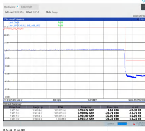
1-N77-3700-3980--30-60-H-6-CP-QPSK-Outer_Full-162@0-Ant1-PASS-see graph
