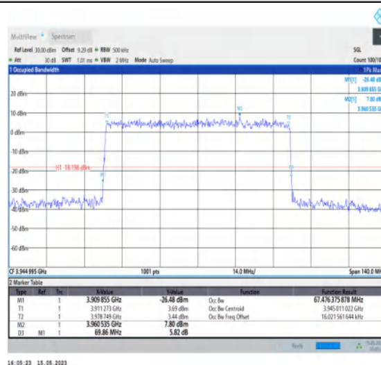
1-N77-3700-3980-PC1-30-70-H-9-CP-256QAM-Outer_Full-189@0-Ant1-67.476-69.860-≤70-PASS
