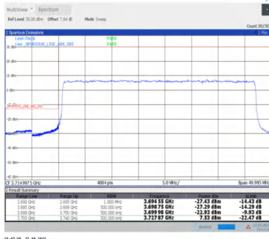
1-N77-3700-3980--30-40-L-3-DFT-PI2BPSK-Outer_Full-100@0-Ant1-PASS-see graph
