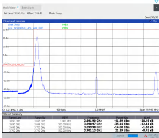
1-N77-3700-3980--30-40-L-4-CP-QPSK-Edge_1RB_L eft-1@0-Ant1-PASS-see graph
