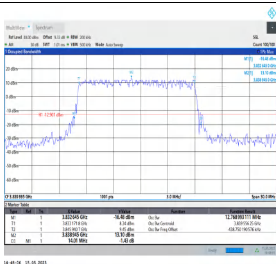
1-N77-3700-3980-PC1-30-15-M-5-DFT-256QAM-Out_er_Full-36@0-Ant1-12.769-14.010-≤15-PASS
