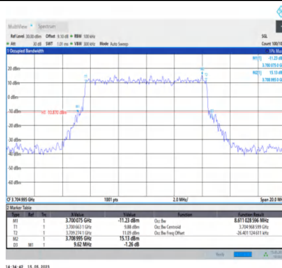
1-N77-3700-3980-PC1-30-10-L-2-DFT-PI2BPSK-Outer_Full-24@0-Ant1-8.611-9.620-≤10-PASS
