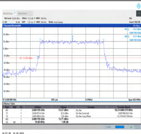
1-N77-3700-3980-PC1-30-20-M-8-CP-64QAM-Outer_Full-51@0-Ant1-18.214-19.480-≤20-PASS
