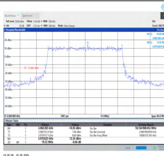
1-N77-3700-3980-PC1-30-20-H-8-CP-64QAM-Outer_Full-51@0-Ant1-18.165-19.520-≤20-PASS
