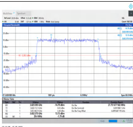
1-N77-3700-3980-PC1-30-30-M-7-CP-16QAM-Outer_Full-78@0-Ant1-27.752-29.400-≤30-PASS
