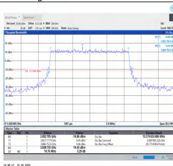
1-N77-3700-3980-PC1-30-15-M-6-CP-QPSK-Outer_Full-38@0-Ant1-13.575-14.760-≤15-PASS
