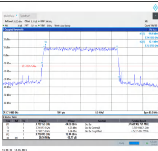
1-N77-3700-3980-PC1-30-40-L-9-CP-256QAM-Outer_Full-106@0-Ant1-37.682-39.760-≤40-PASS
