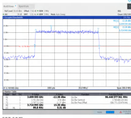
1-N77-3700-3980--30-100-L-2-DFT-P12BPSK-Outer_Fu Full-270@0-Ant1-96.448-99.800-≤100-PASS
