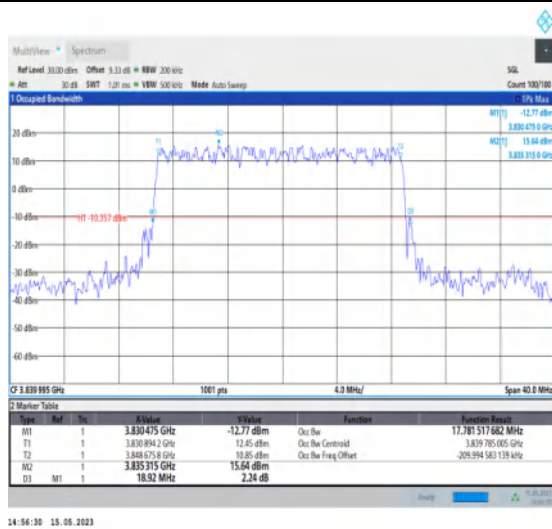
1-N77-3700-3980-PC1-30-20-M-2-DFT-PI2BPSK-Out_Full-50@0-Ant1-17.782-18.920-≤20-PASS
