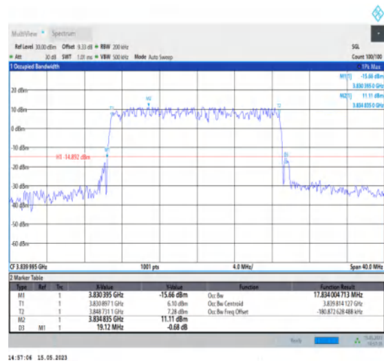
1-N77-3700-3980-PC1-30-20-M-5-DFT-256QAM-Out_Full-50@0-Ant1-17.834-19.120-≤20-PASS
