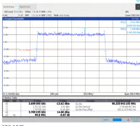
1-N77-3700-3980--30-100-L-1-DFT-QPSK-Outer_Fu II-270@0-Ant1-96.336-99.800-≤100-PASS
