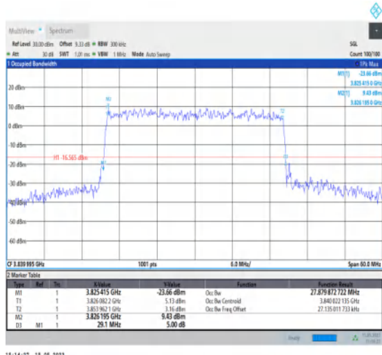
1-N77-3700-3980-PC1-30-30-M-9-CP-256QAM-Outer_Full-78@0-Ant1-27.88-29.100-≤30-PASS
