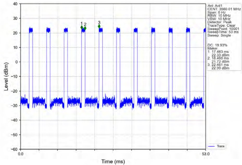
n48_30kHz_SISO_NTNV_20MHz_CP-OFDM_64_QAM_3560.01MHz_Inner_Full_Ant1
