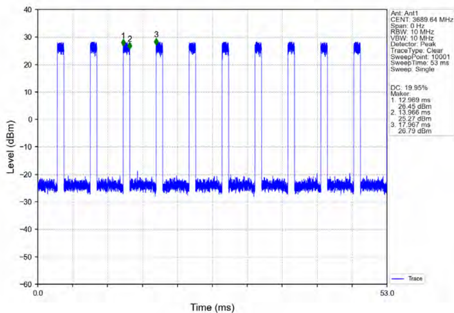
n48_30kHz_SISO_NTNV_20MHz_CP-OFDM_64_QAM_3690MHz_Inner_Full_Ant1
