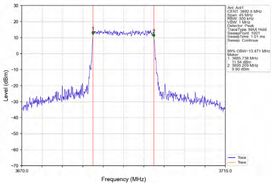
Band48_15MHz_16QAM_HCH_3692.5MHz_RB_75_0_NTNV
