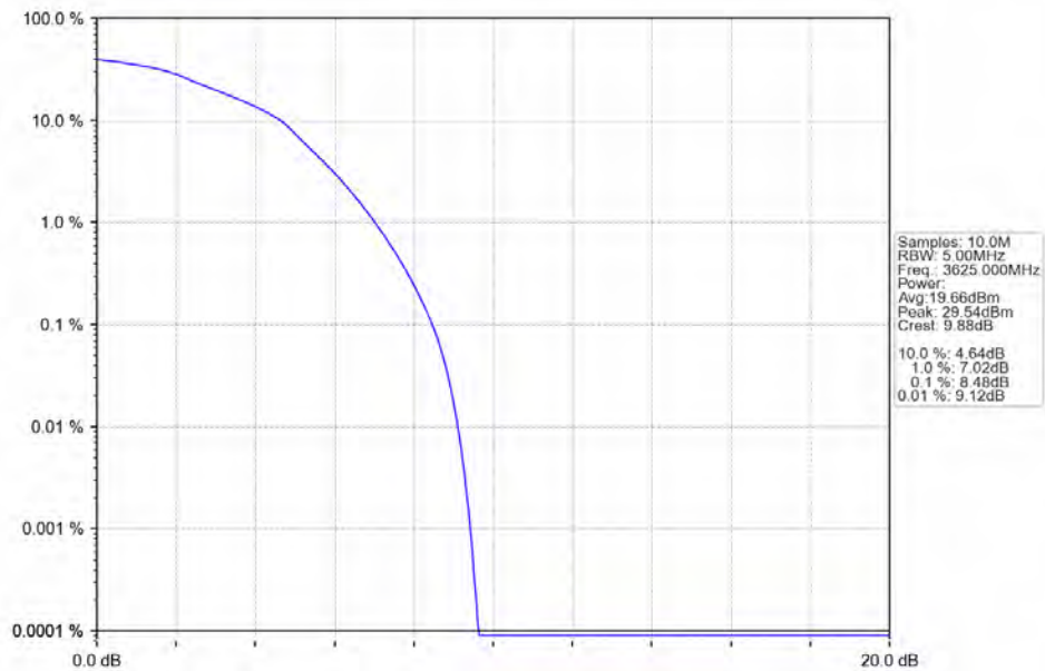
Band48_5MHz_64QAM_MCH_3625MHz_RB_25_0_NTNV
