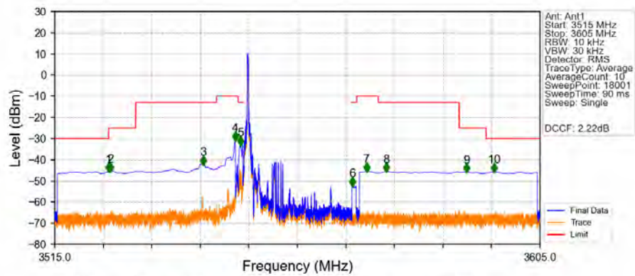
Band48_15MHz_QPSK_LCH_3557.5MHz_RB_1_0_NTNV
