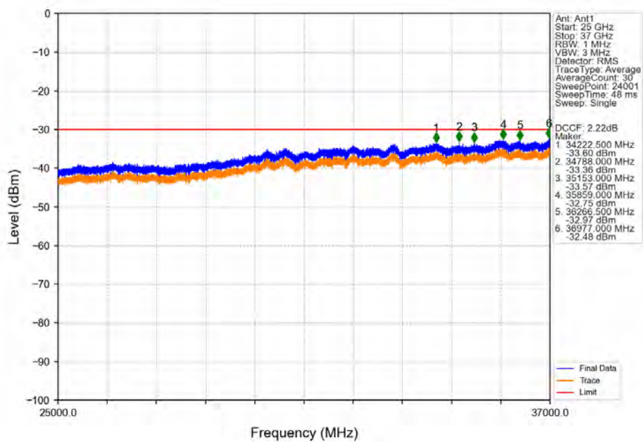
Band48_5MHz_16QAM_LCH_3552.5MHz_RB_1_0_NTNV
