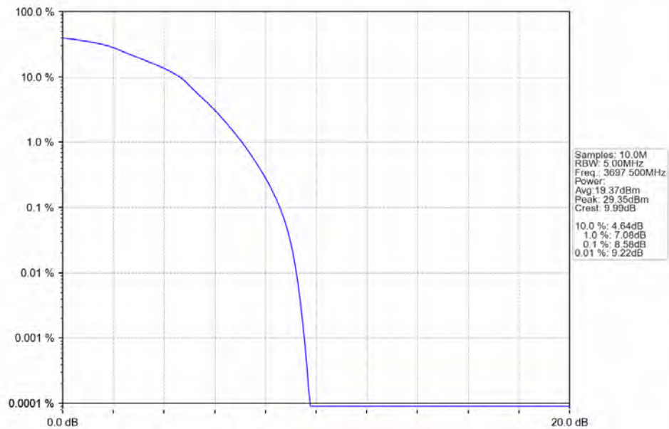
Band48_5MHz_16QAM_HCH_3697.5MHz_RB_25_0_NTNV
