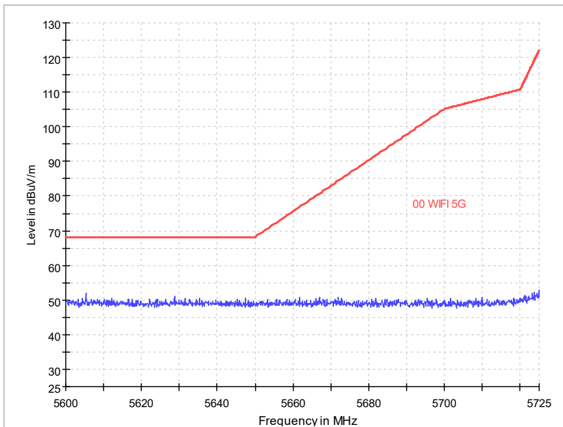
Radiated Emission Band Edge Channel No.:149 Test Mode: 802.11a Polarization: V
