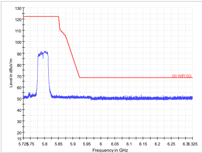
Radiated Emission Band Edge Channel No.:159 Test Mode: 802.11ac Polarization: V
