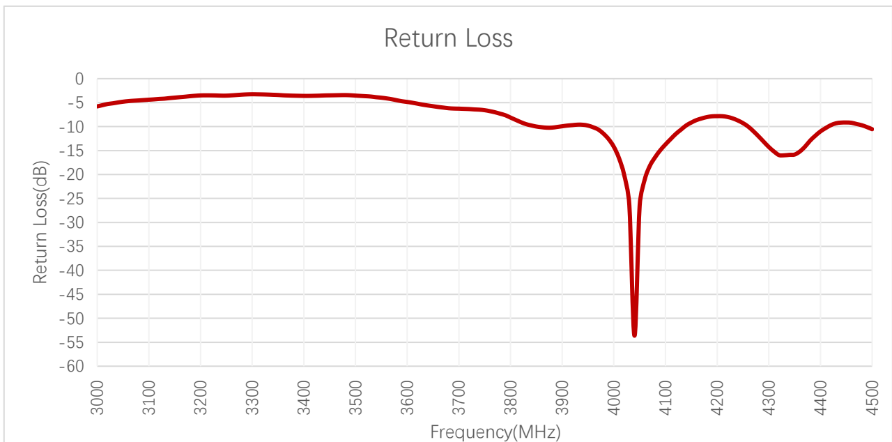
Return Loss (dB)
