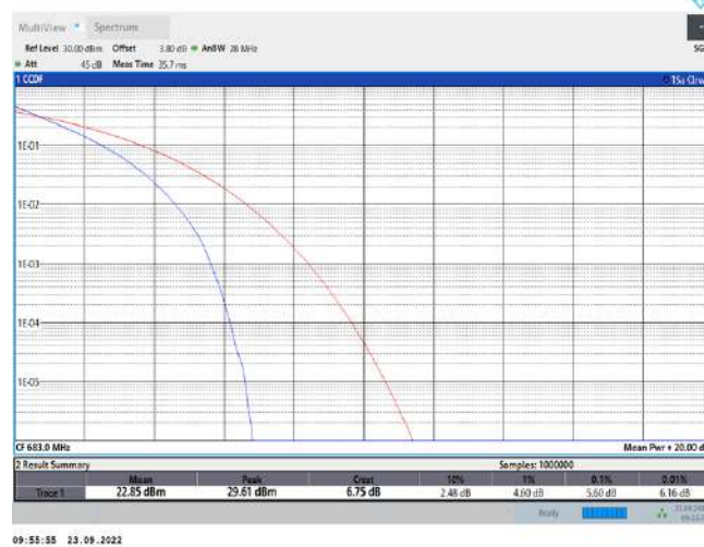
Band71-20MHz-QPSK-133322-100RB#0
