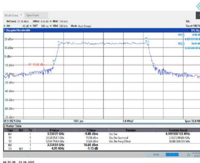
Band48-5MHz-QPSK-55990-25RB#0
