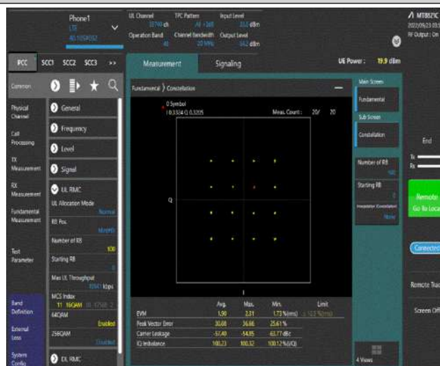
Band48-20MHz-16QAM-55740-100RB#0
