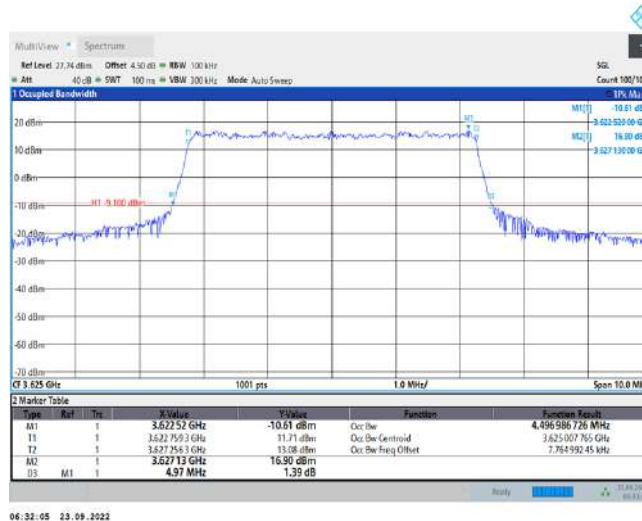
Band48-5MHz-QPSK-55990-25RB#0
