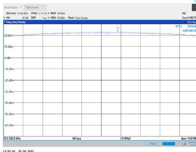
Band48-5MHz-QPSK-55265-1RB#12
