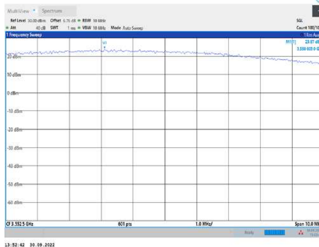
Band48-5MHz-QPSK-55265-1RB#12
