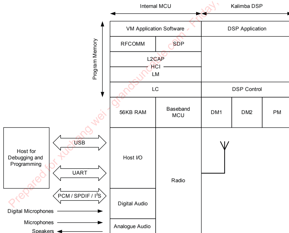
Figure 18.1: Stand-alone CSR8670 WLCSP and Kalimba DSP Applications
