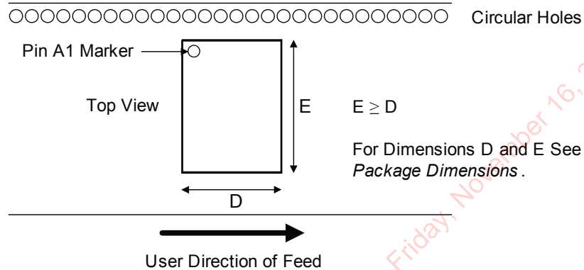
Figure 19.1: Tape Orientation
