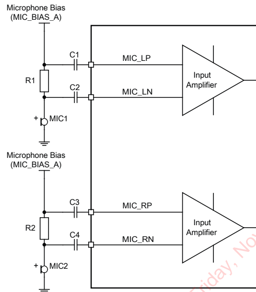
Figure 9.6: Microphone Biasing
