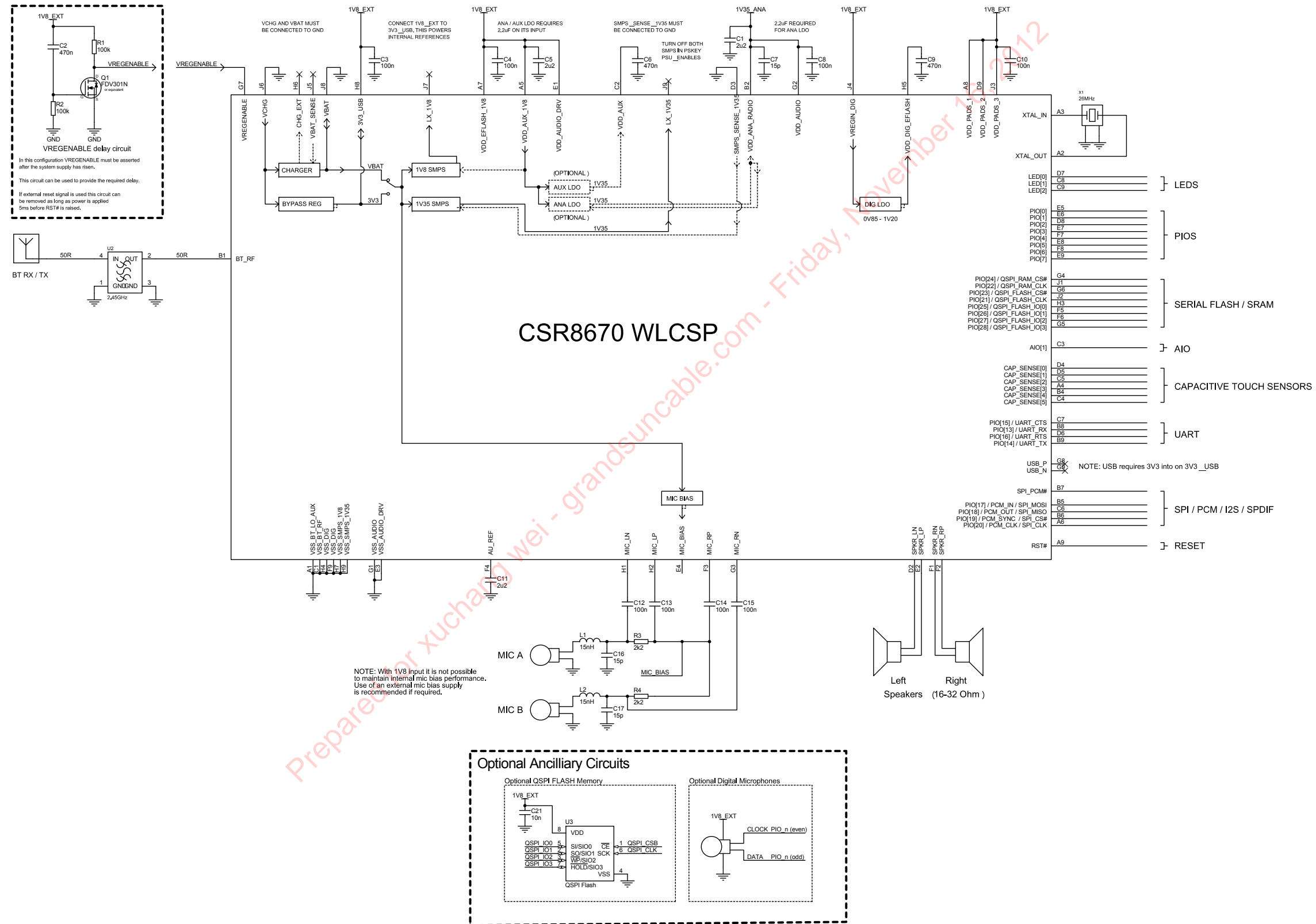
Figure 14.1: External 1.8V Supply Example Application
