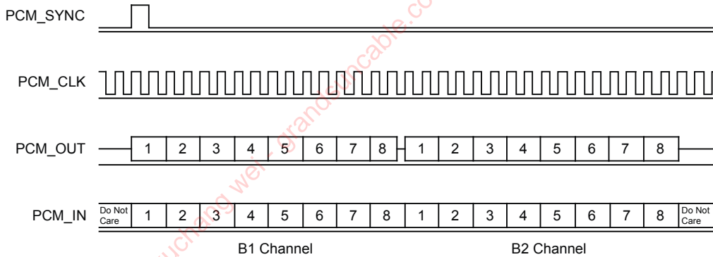
Figure 9.16: GCI Interface
