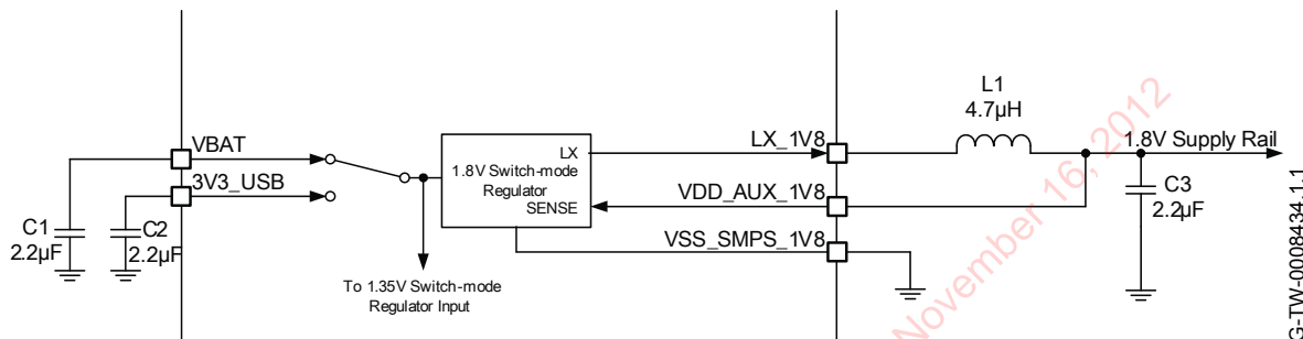
Figure 11.4: 1.8V Switch-mode Regulator Output Configuration
