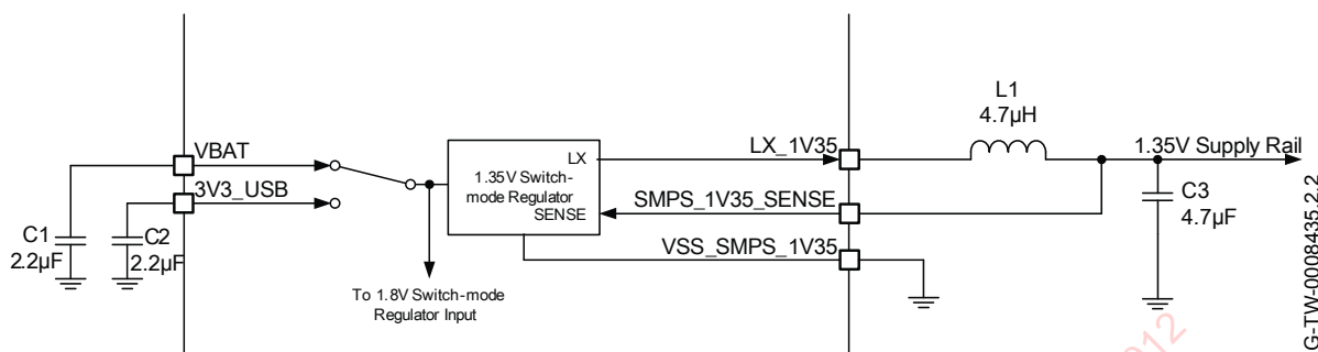
Figure 11.5: 1.35V Switch-mode Regulator Output Configuration
