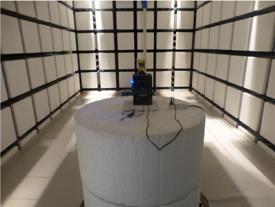
Transmitting mode (Above 1GHz)
