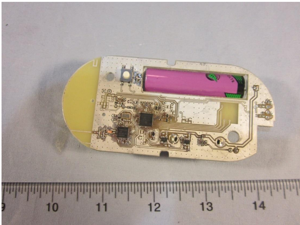
VSW1301 Sensor, Circuit Board Bottom View Scale, Horizontal
