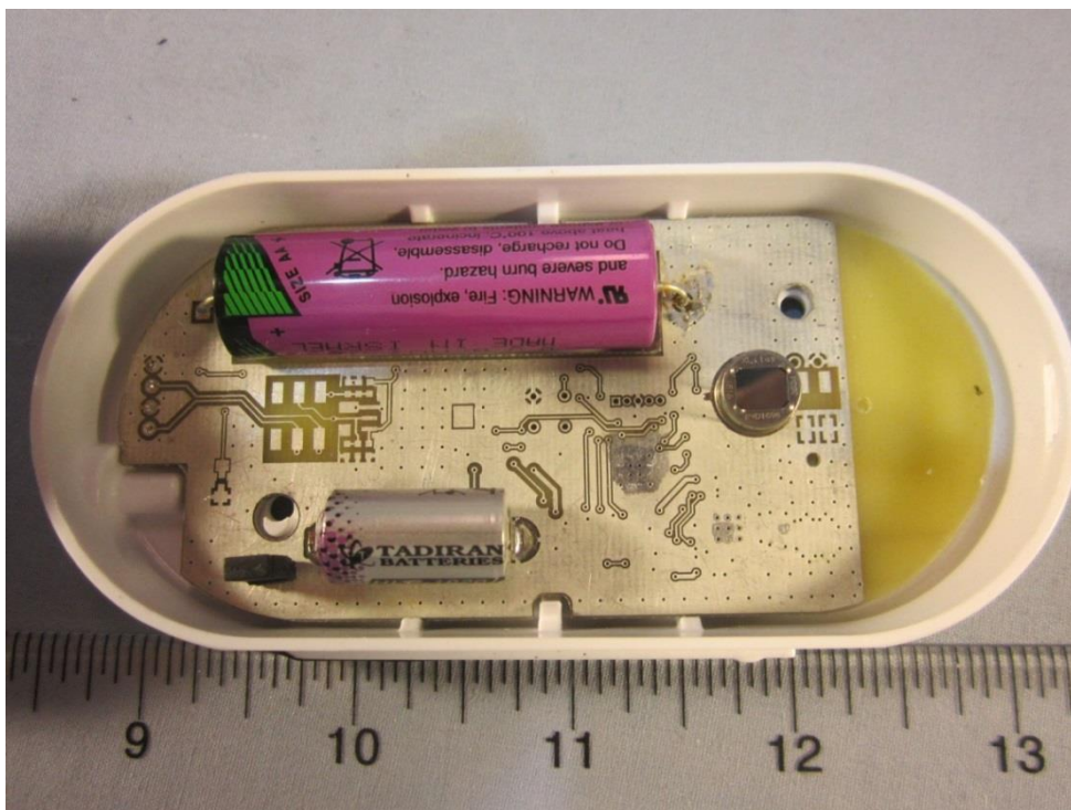
VSW1301 Sensor, Top Cover Removed View Scale, Horizontal
