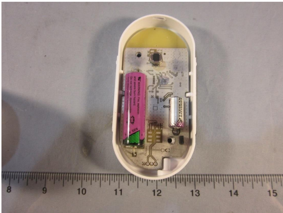
VSW1301 Sensor, Top Removed, Rotated 180 deg. View Scale, Vertical
