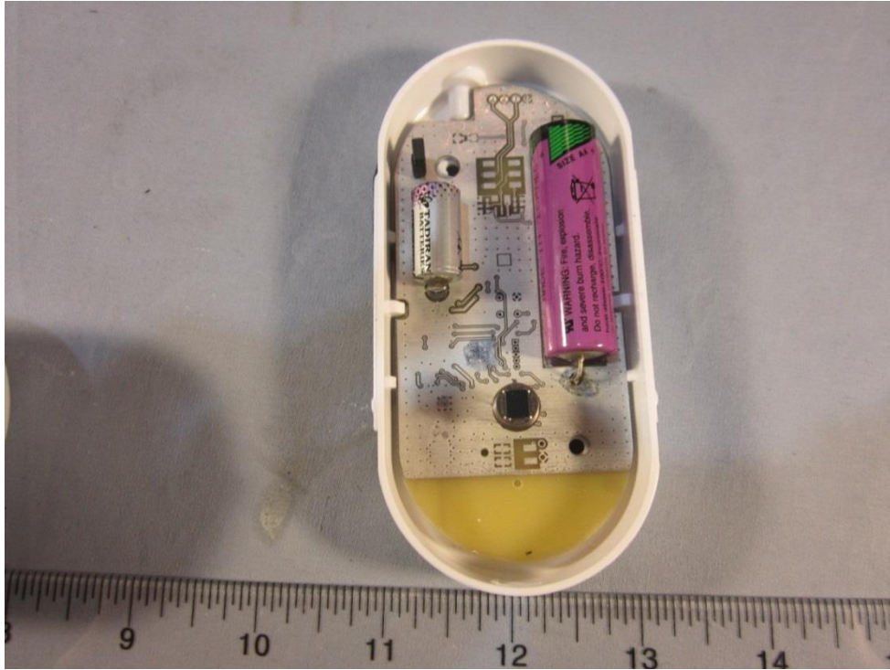
VSW1301 Wall Mount Occupancy/Vacancy Sensor, Top View Scale, Vertical
