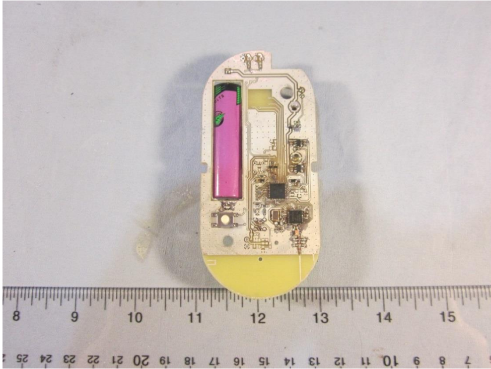
VSW1301 Wall Mount Occupancy/Vacancy Sensor, Circuit Board Bottom View Scale, Vertical
