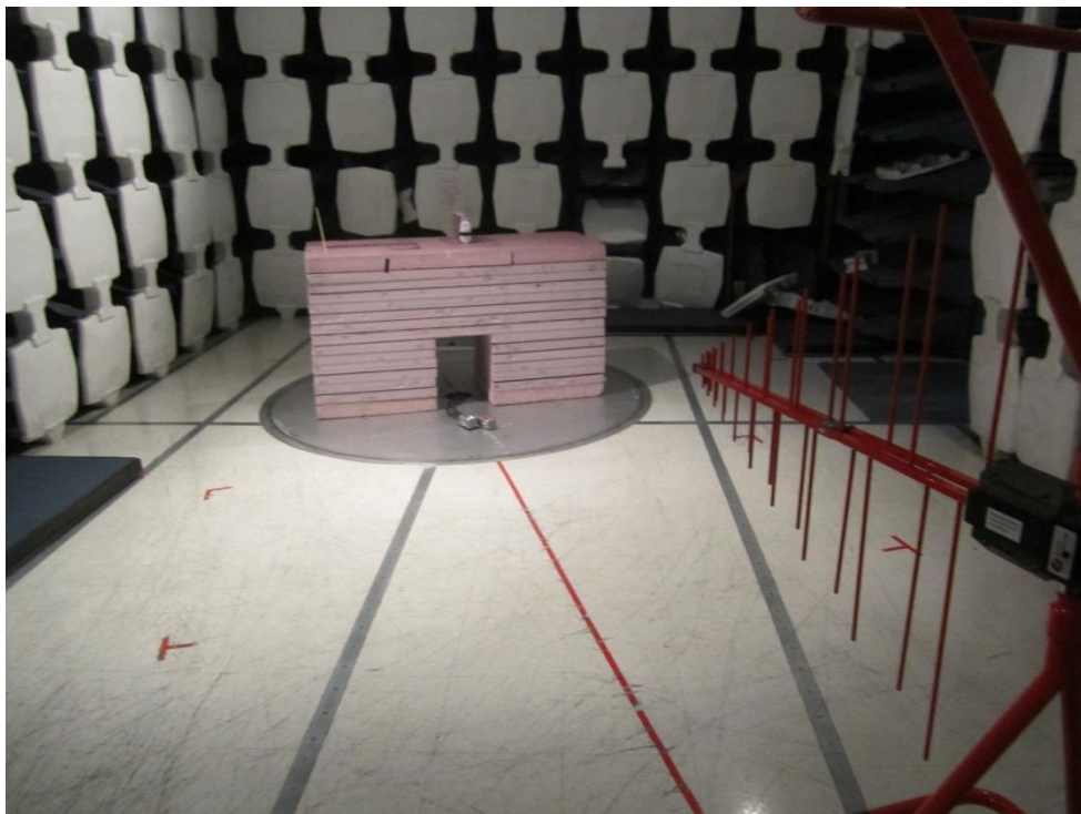
Radiated Emissions 30-1000MHz Front View
