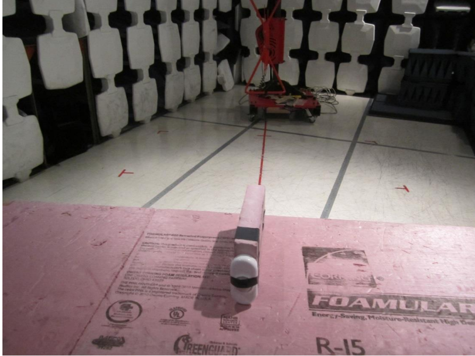
Radiated Emissions 30-1000MHz Rear view
