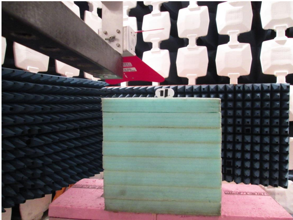
Radiated Emissions 6-10GHz Front View
