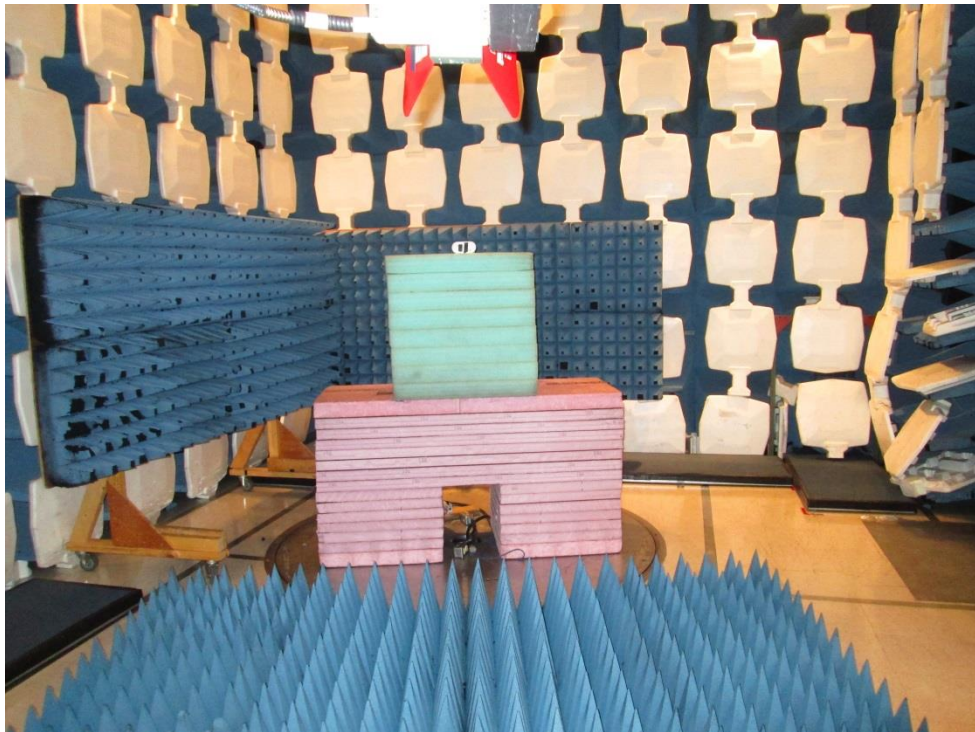
Radiated Emissions 1-6GHz Front View
