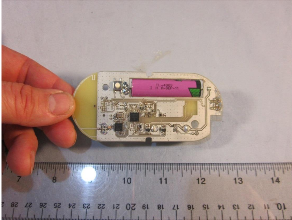
VSC1302 Ceiling Mount Occupancy/Vacancy Sensor, Circuit Board Scale Bottom View, Horizontal
