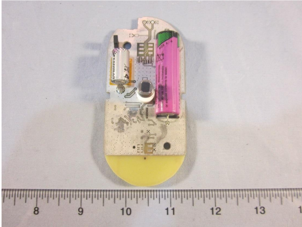
VSC1302 Ceiling Mount Occupancy/Vacancy Sensor, Circuit Board Scale Top View, Vertical
