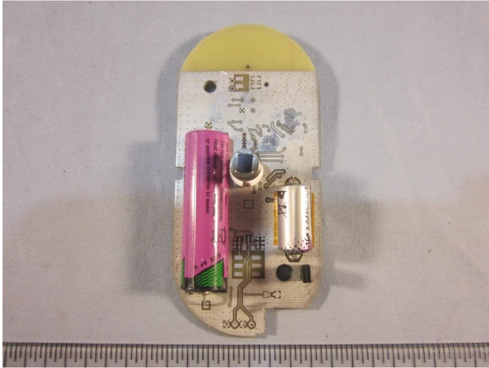
VSC1302, Ceiling Mount Occupancy/Vacancy Sensor, Vertical Top View
