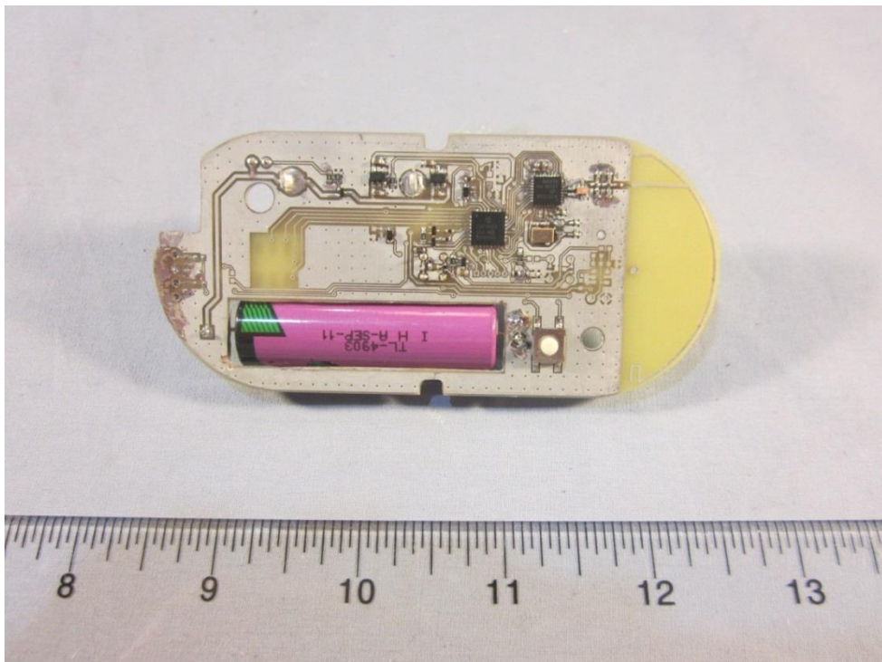
VSC1302 Sensor, Circuit Board Scale Bottom View, Horizontal
