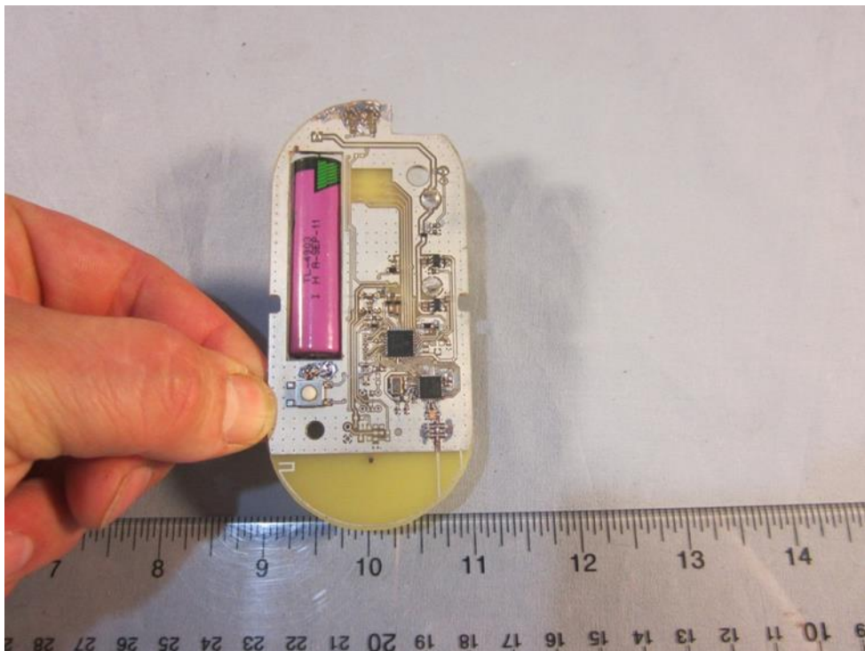
VSC1302 Sensor, Circuit Board Scale Bottom View, Vertical
