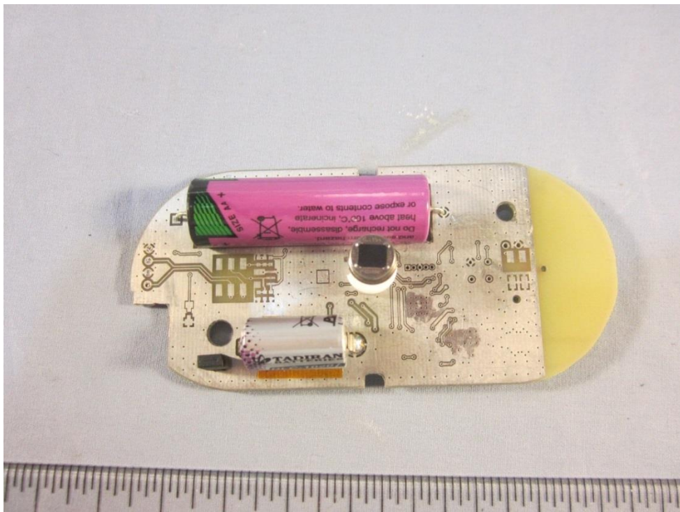
VSC1302, Ceiling Mount Occupancy/Vacancy Sensor, Circuit Board Top View
