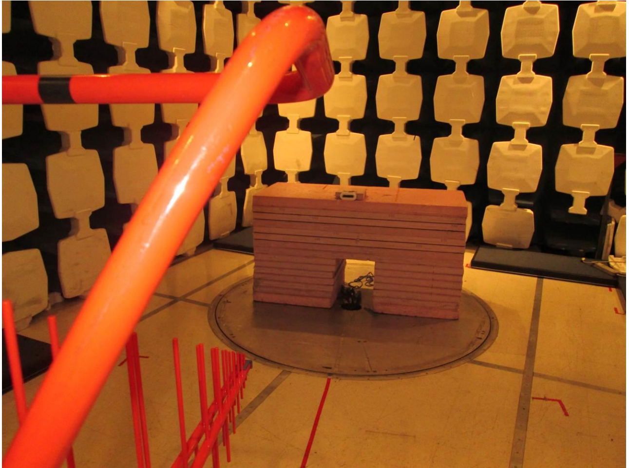
Radiated Emissions - 30 to 1000 MHz
