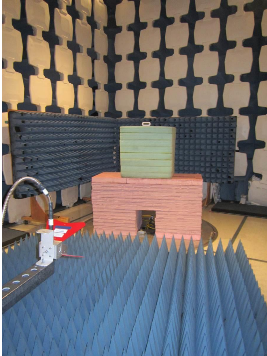
Radiated Emissions - 1 to 6 GHz
