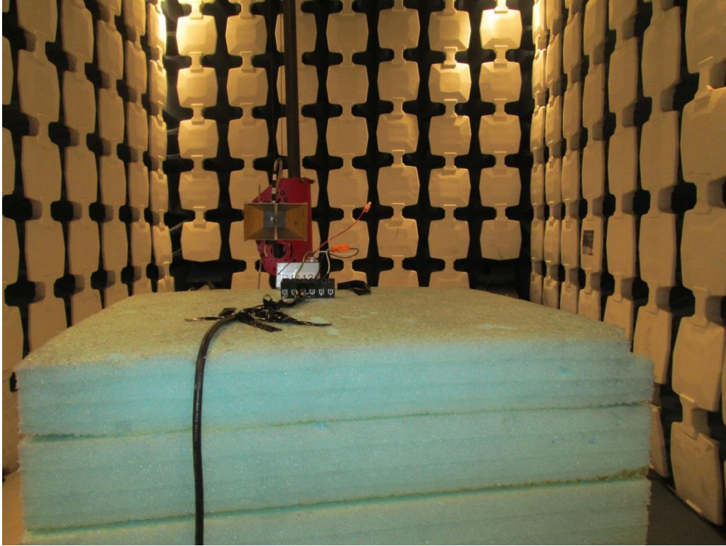
6-10GHz – Rear
