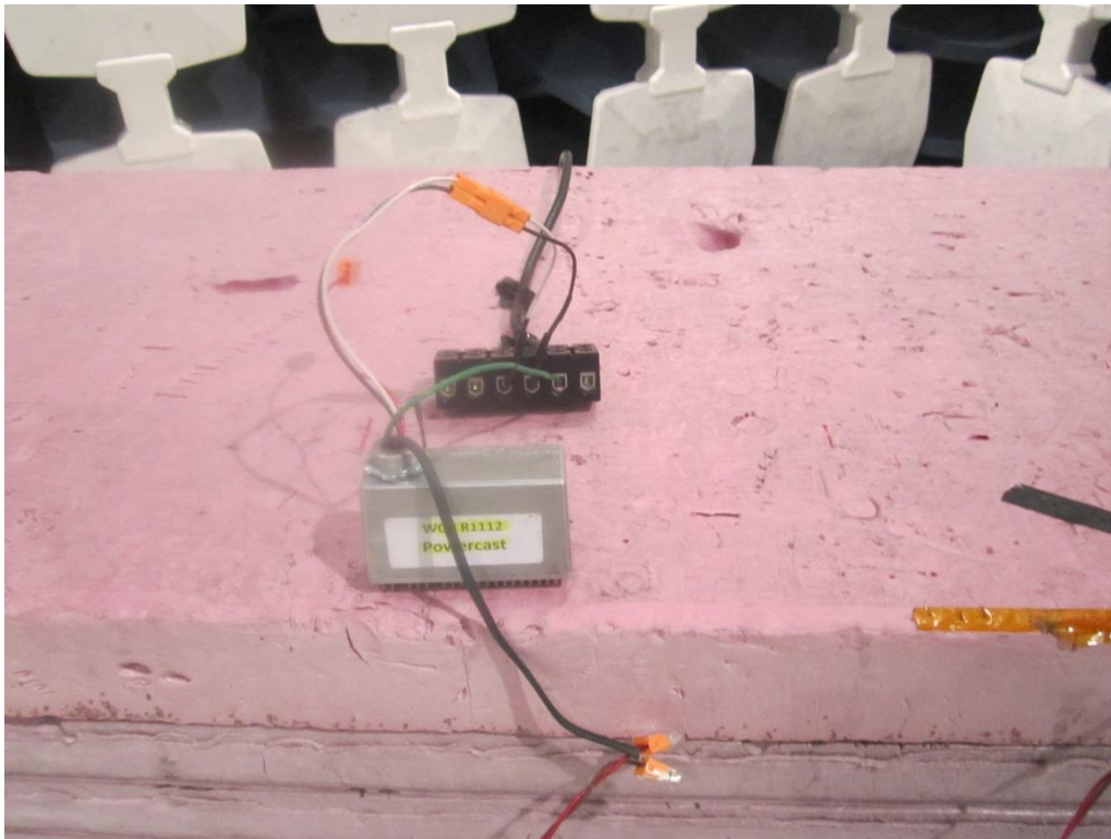
Radiated Emissions Test Y-Axis Close-Up View
