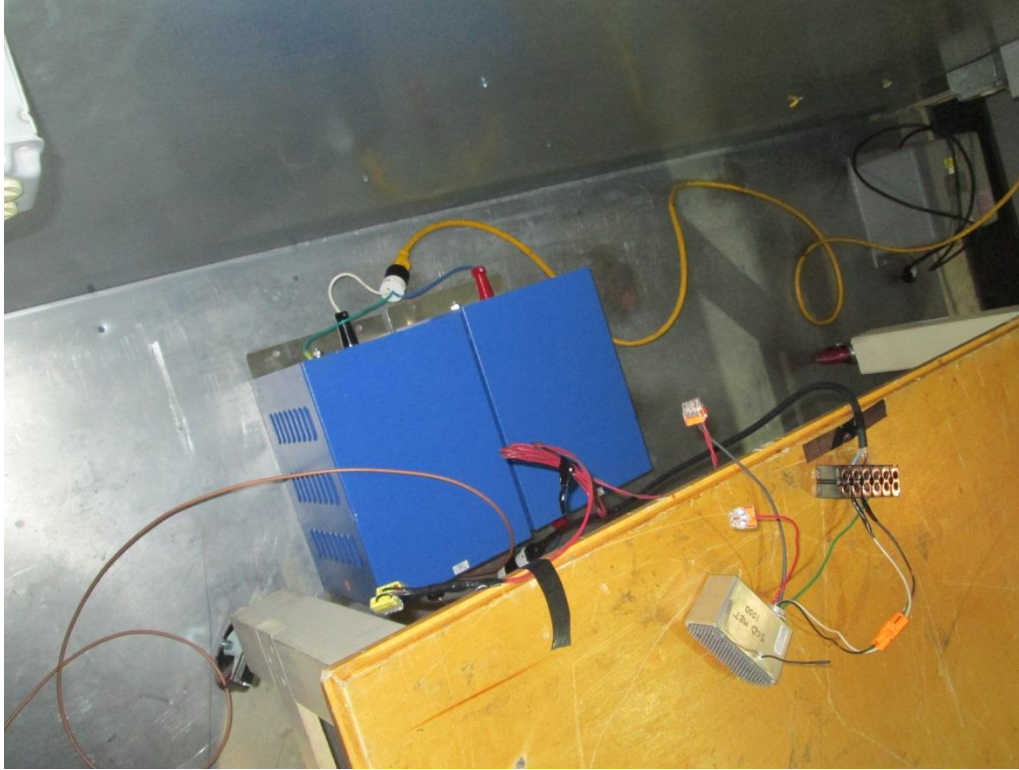
Conducted Emissions Test 115 Volt AC Top View
