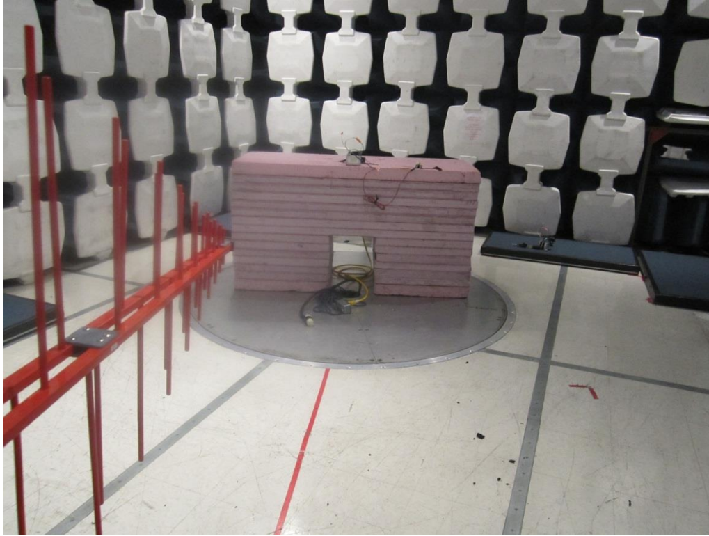
REMI Test Front View
