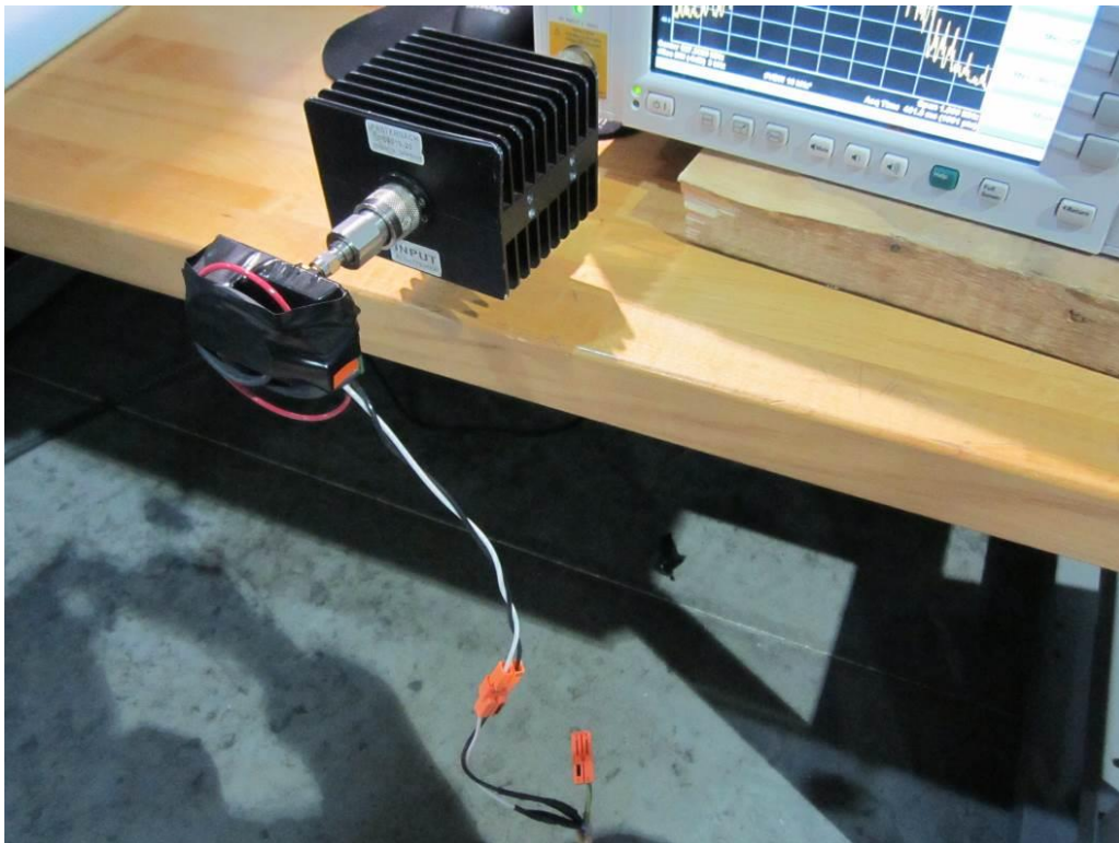
Conducted Testing at Antenna port (Close-up View)
