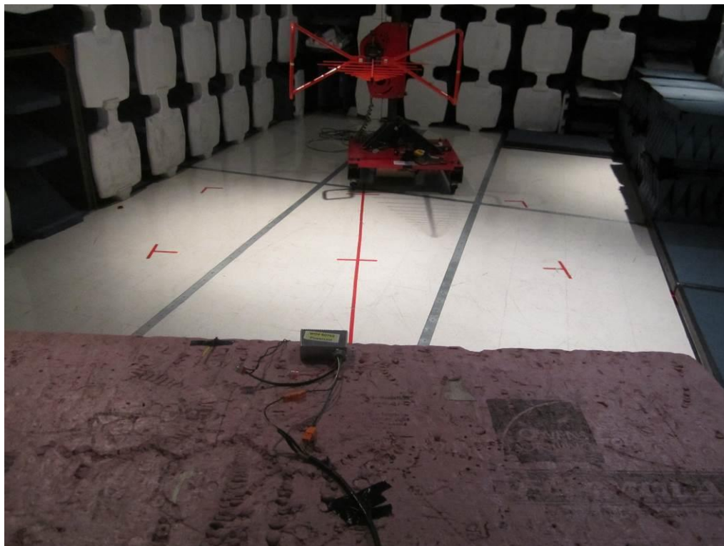
Radiated Emissions – 30MHz to 1GHz
