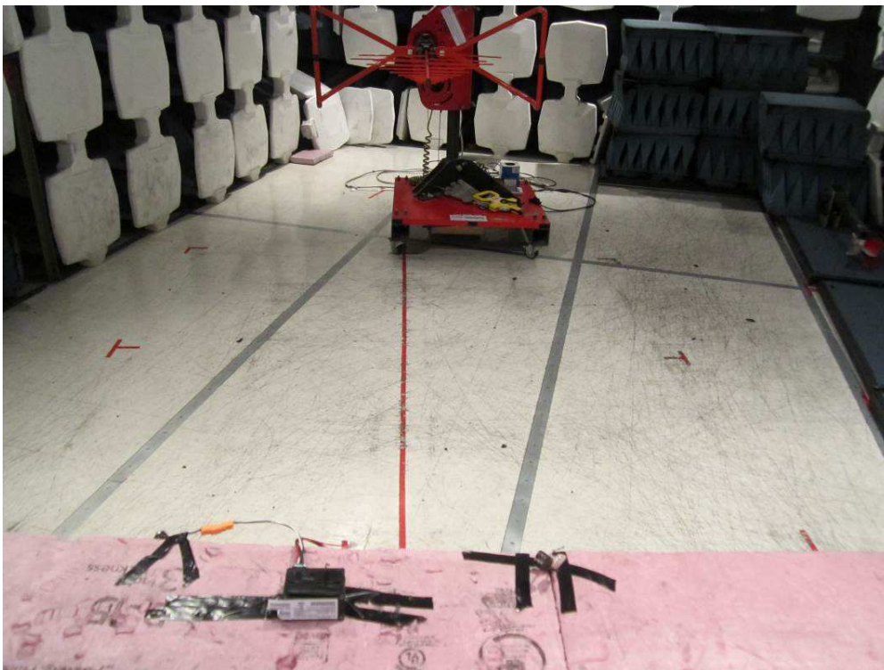
Radiated Emissions – Mid range (X orientation)
