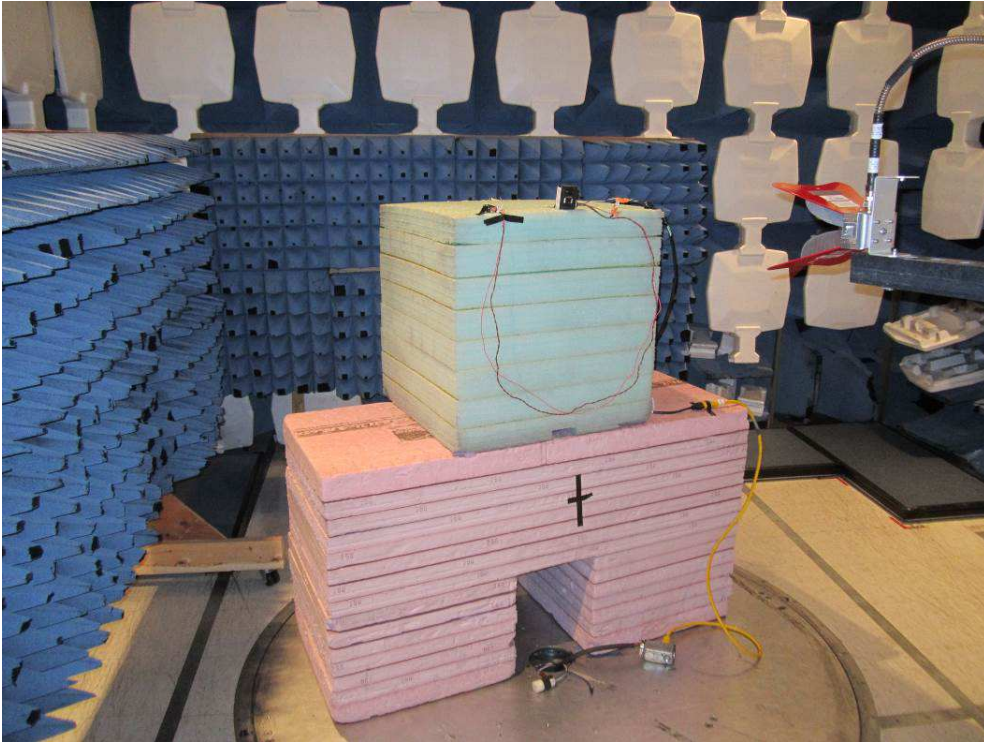
Radiated Emissions – 6 to 10 GHz
