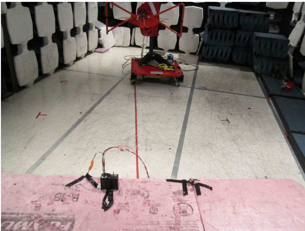
Radiated Emissions – Mid range (Y orientation)
