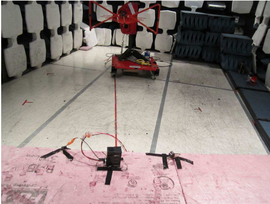
Radiated Emissions – Mid range (Z orientation)
