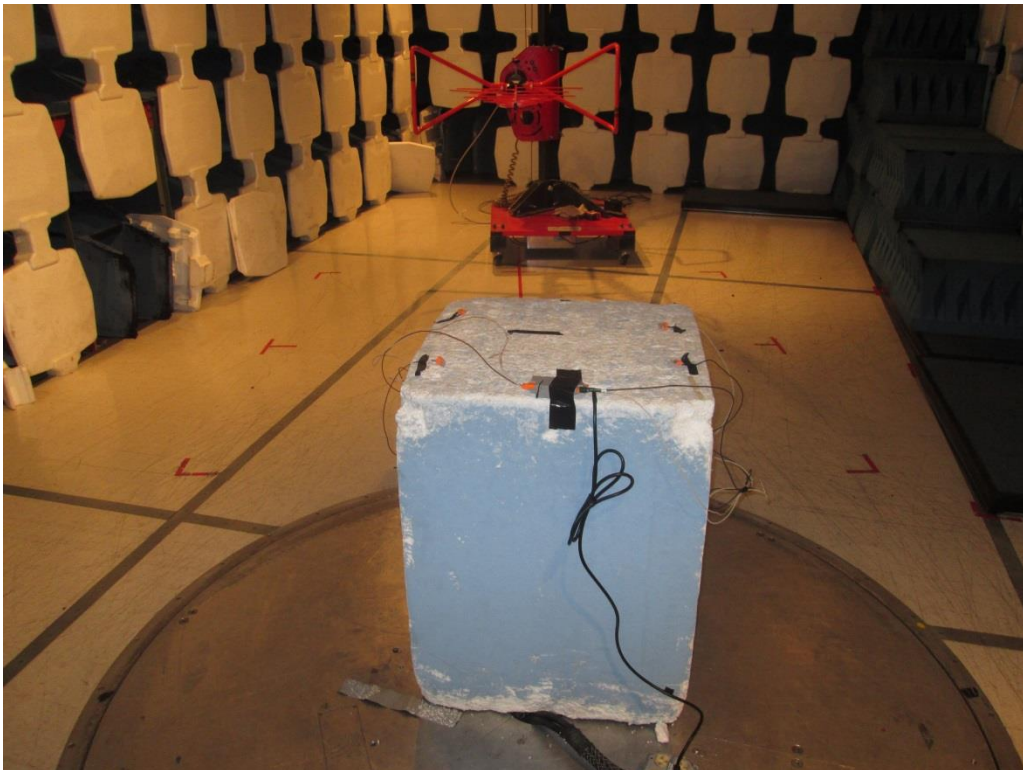
EMI Radiated Spurious – 30 to 1000MHz
