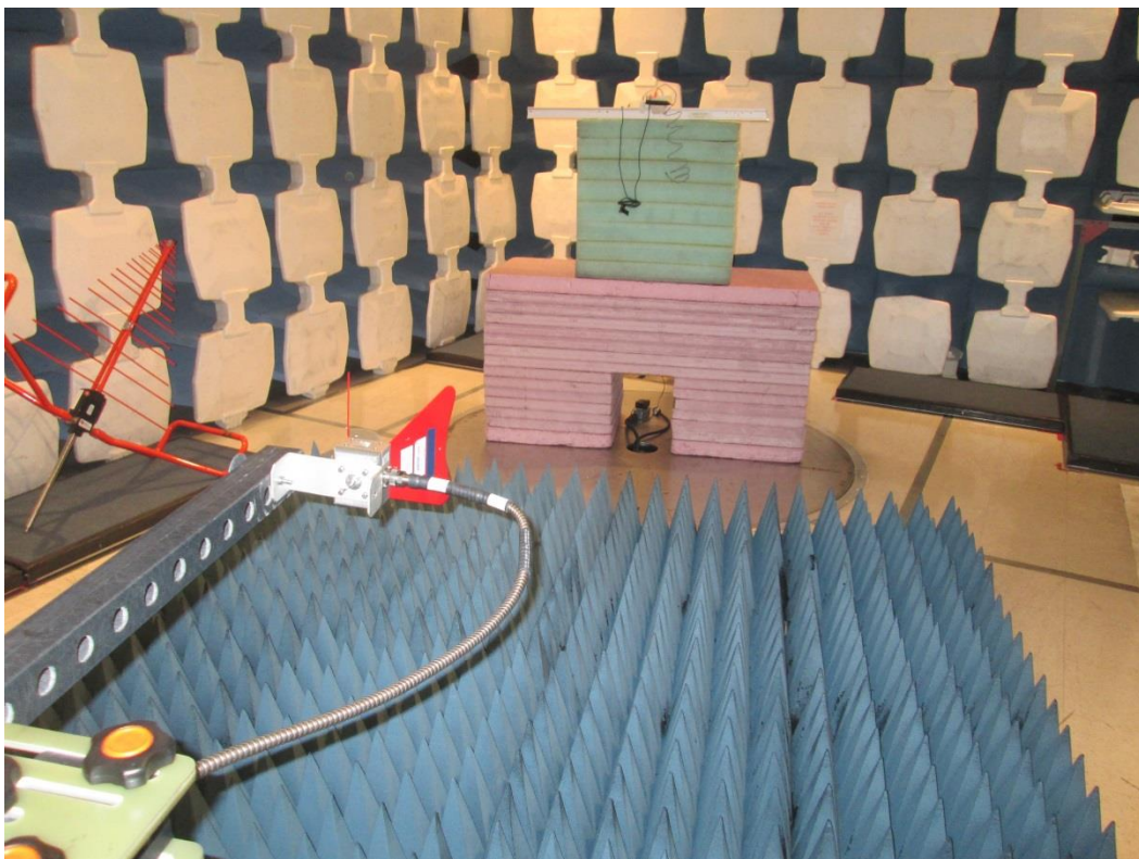
Radiated Spurious Emissions (1GHz – 6GHz)
