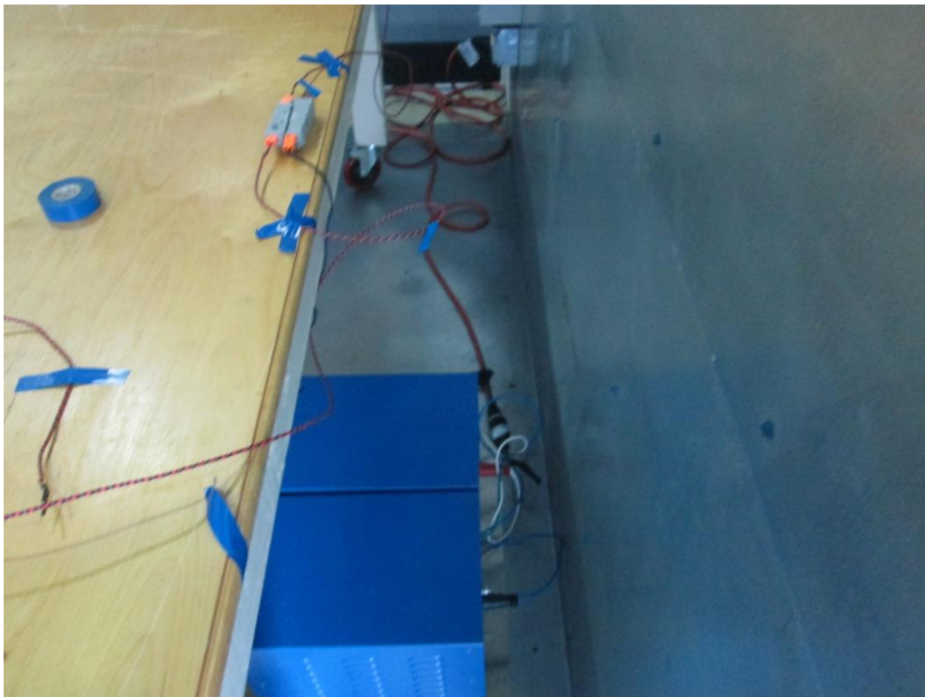
EMI Conducted – AC Mains (Rear – 0.15 to 30 MHz)
