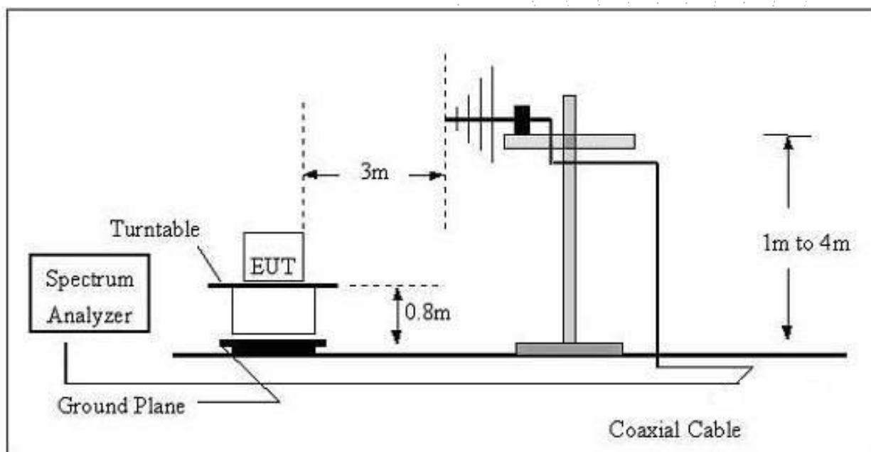
(B) Radiated Emission Test-Up Frequency 30MHz~1GHz
