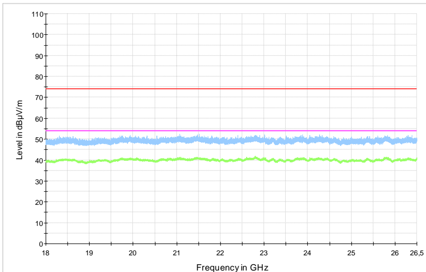
— Preview Result 2-AVG ★ Critical_Freqs AVG — FCC_15C_15.209_Radiated Emissions_Peak ◆ Final_Result PK+ — Preview Result 1-PK+ ★ Critical_Freqs PK+ — FCC_15C_15.209_Radiated Emissions_Avg ◆ Final_Result AVG
