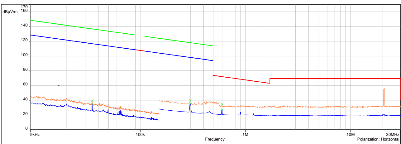
Parallel Polarization_9kHz to 30 MHz
