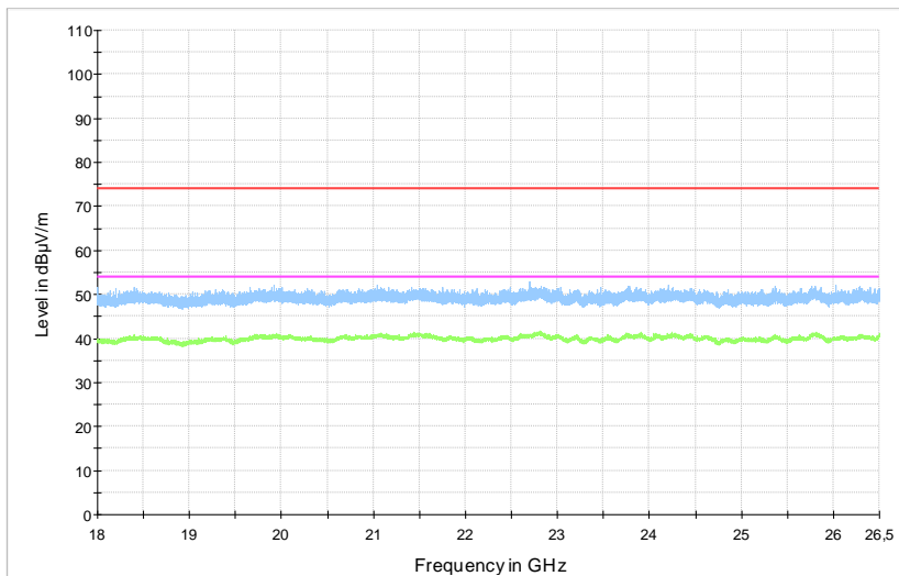
— Preview Result 2-AVG ★ Critical_Freqs AVG — FCC_15C_15.209_Radiated Emissions_Peak ★ Critical_Freqs PK+ — Preview Result 1-PK+ — FCC_15C_15.209_Radiated Emissions_Avg ◆ Final_Result PK+ ◆ Final_Result AVG
