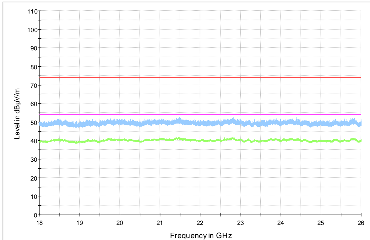
— Preview Result 2-AVG — Preview Result 1-PK+ — FCC_15C_15.209_Radiated Emissions_Peak — FCC_15C_15.209_Radiated Emissions_Avg ◆ Final_Result PK+ ◆ Final_Result AVG
