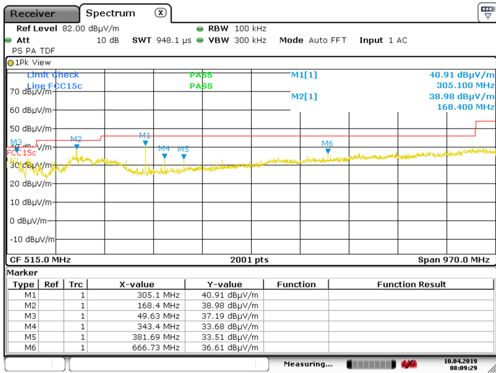
Plot of the emissions (Peak detector values shown) M1, M2, M3 are from the AUX1 (laptop)
