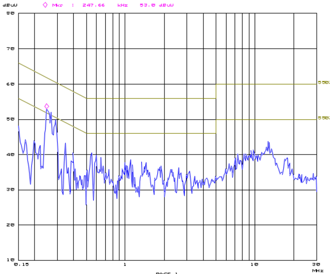
Plot of the AC Power-line Conducted emissions N, @2402 MHz
