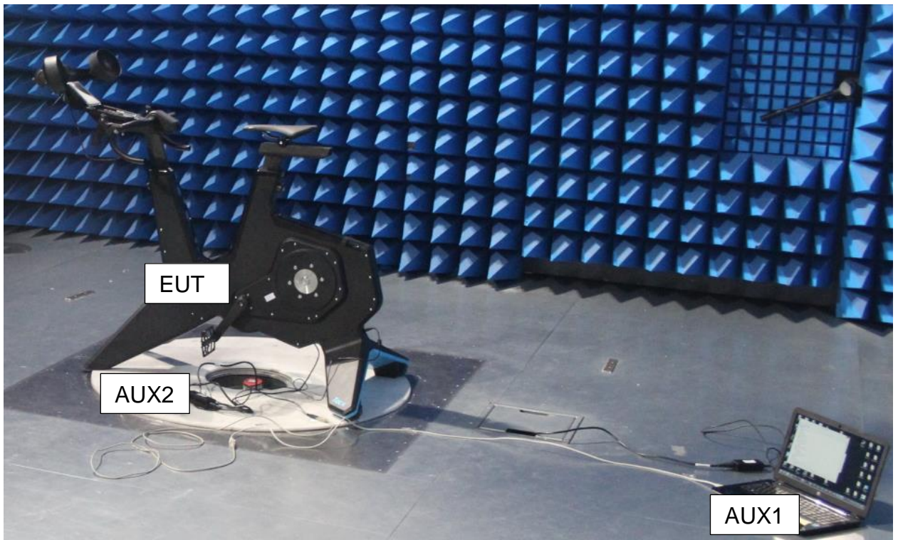
Figure 3c: Test Setup Photos – radiated tests and programming
