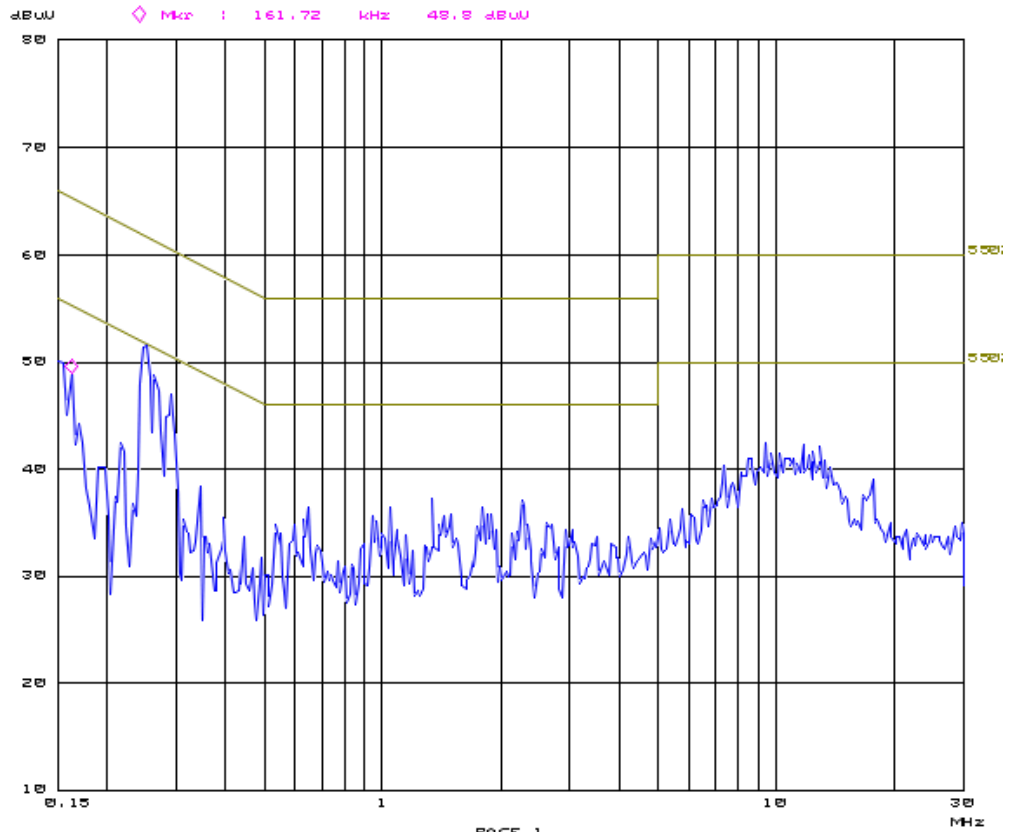
Plot of the AC Power-line Conducted emissions on L1, @2402 MHz
