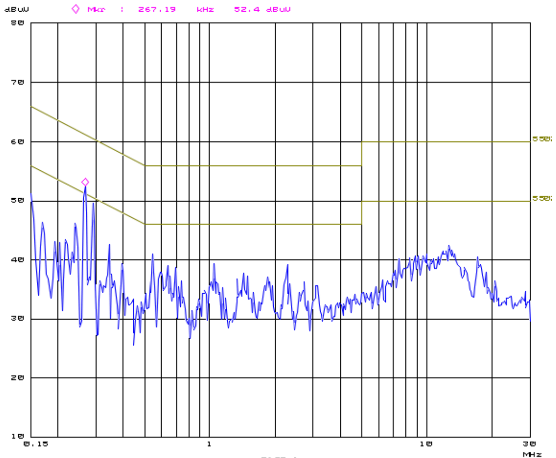
Plot of the AC Power-line Conducted emissions N, @2440 MHz
