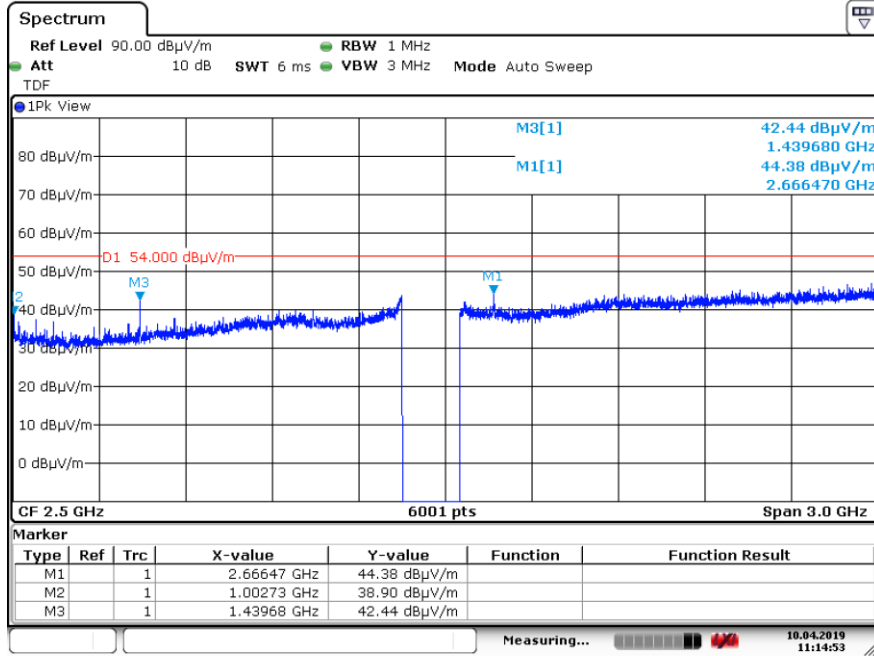
Plot of the emissions at 2402 MHz, Vertical polarization, Peak values shown gap in the plot is of the used Notch filter
