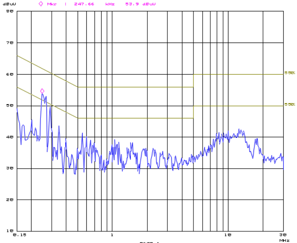
Plot of the AC Power-line Conducted emissions N, @2480 MHz
