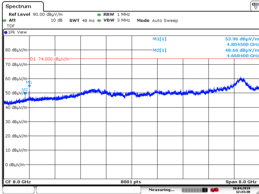
Plot of the emissions at 2402 MHz, range 4 to 12 GHz, Vertical polarization, Peak values shown
