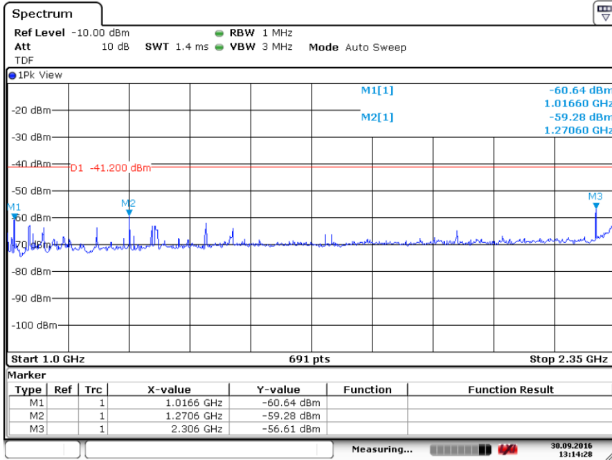
Plot of the emissions at 2403 MHz, Vertical polarization, Peak values shown
