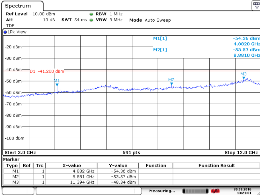
Plot of the emissions at 2442 MHz, Vertical polarization, Peak values shown
