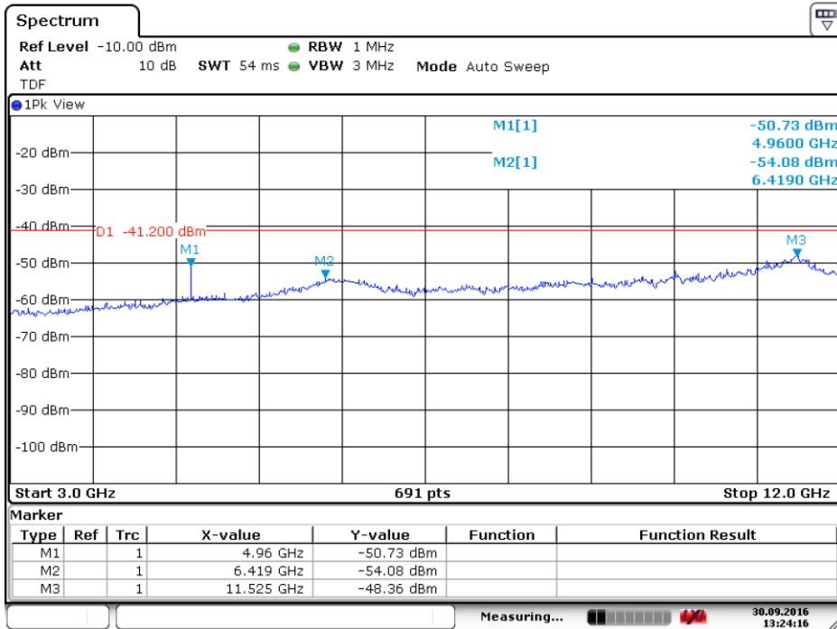
Plot of the emissions at 2480 MHz, Vertical polarization, Peak values shown
