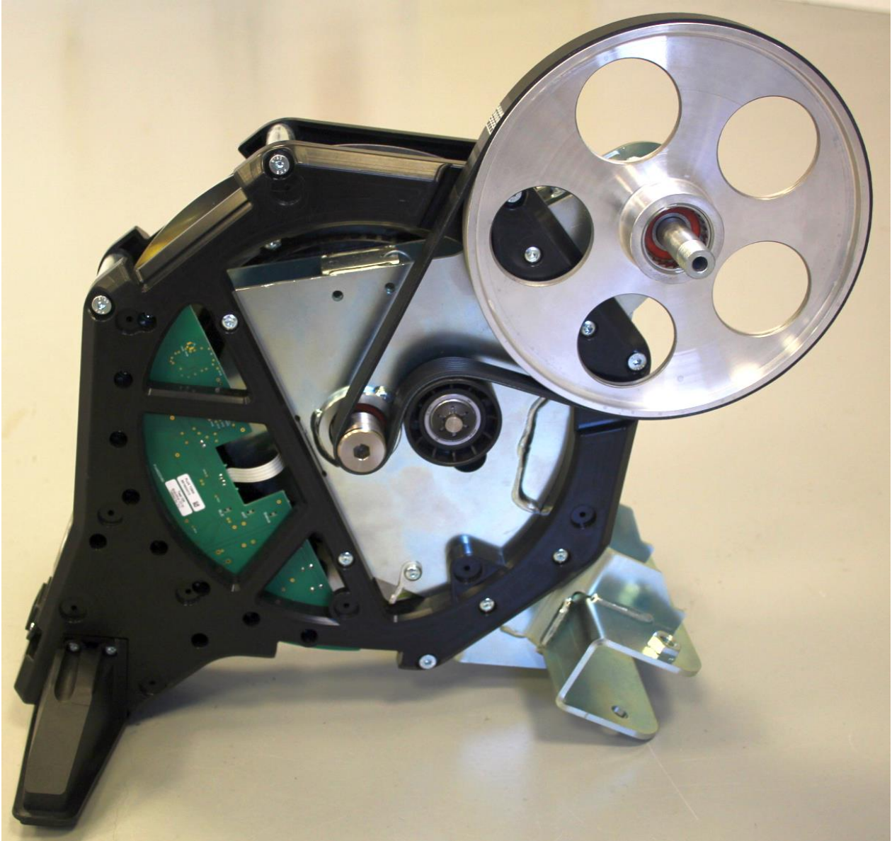
Left side, holding the transmitters (cover removed)
