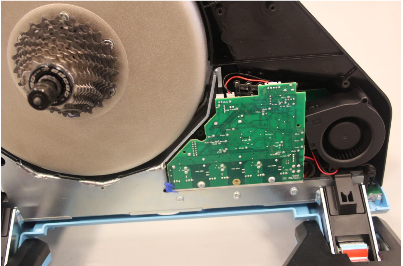
Left side, holding the transmitters (cover removed)
