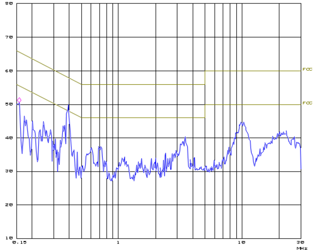
Plot of the AC Power-line Conducted emissions with AUX2a on N
