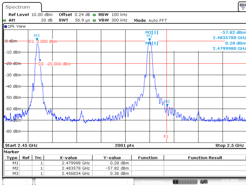
Plot: Band Edge Conducted Emission, Spectral Diagram, Normal mode. Plot showing more than 20 dB band edge attenuation. F1 shows the band edge frequency of 2483.5 MHz.
