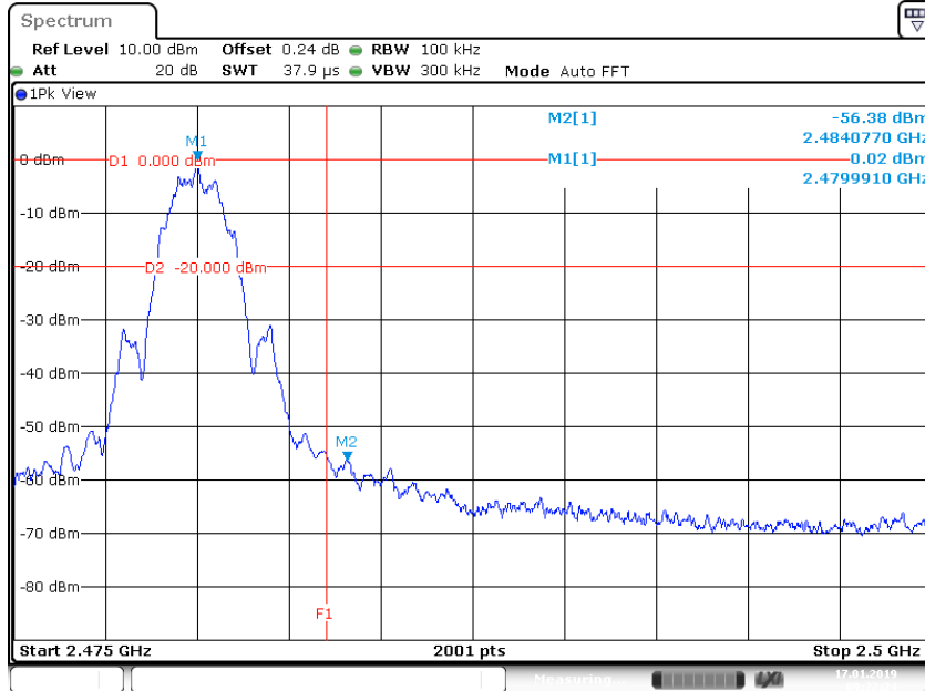
Plot: Band Edge Conducted Emission, Spectral Diagram, 2480 MHz. Plot showing more than 20 dB band edge attenuation. F1 shows the band edge frequency of 2483.5 MHz.
