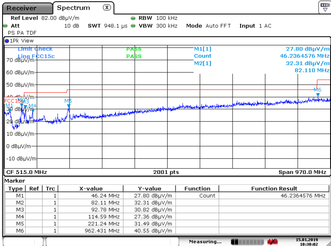
Plot of the emissions (Peak detector values shown)
