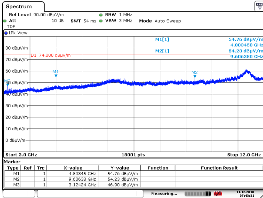
Plot of the emissions at 2402 MHz, Vertical polarization, Peak values shown
