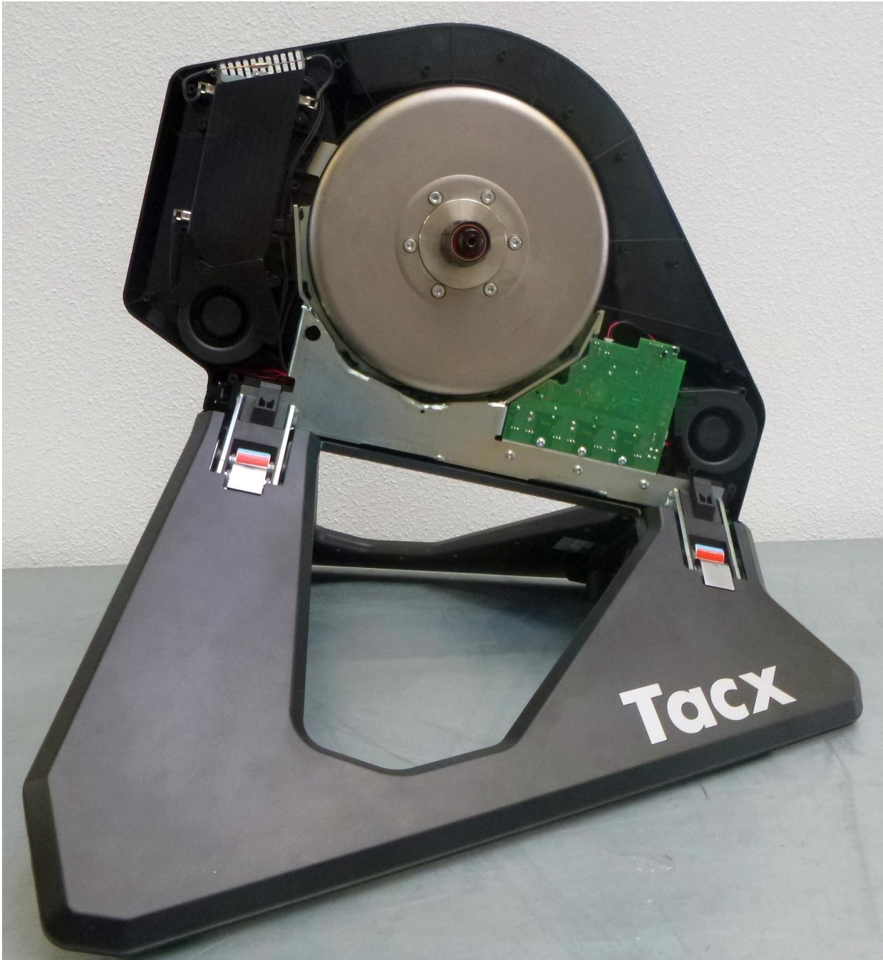
Left side, holding the transmitters (cover removed)
