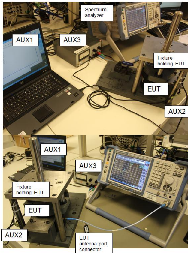
Photo 1: basic setup for frequency programming
