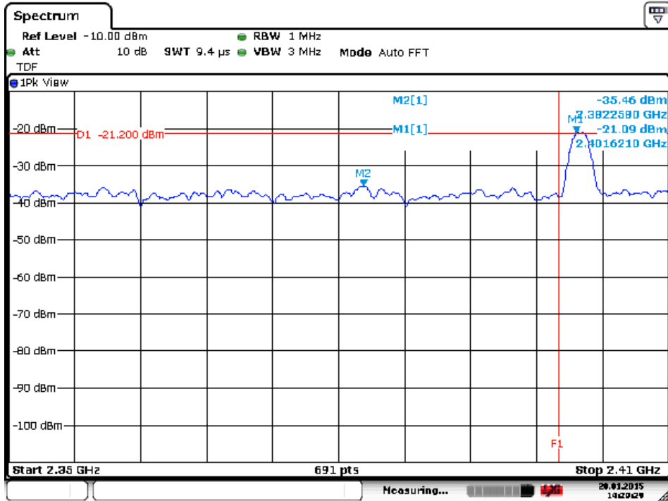
Plot 1a Peak value
