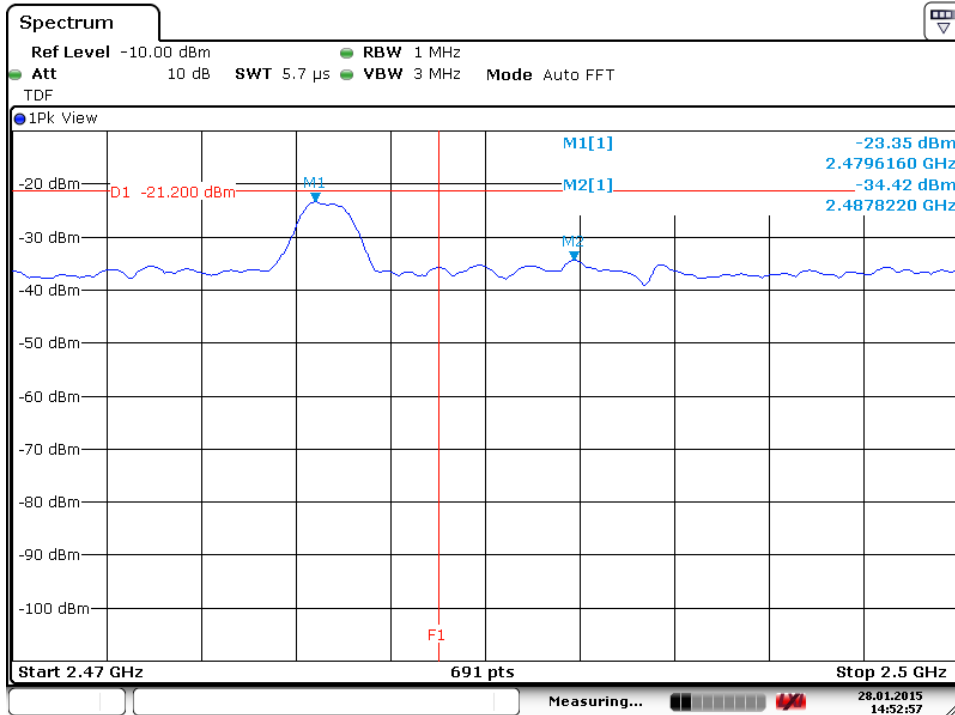
Plot 2a Peak value
