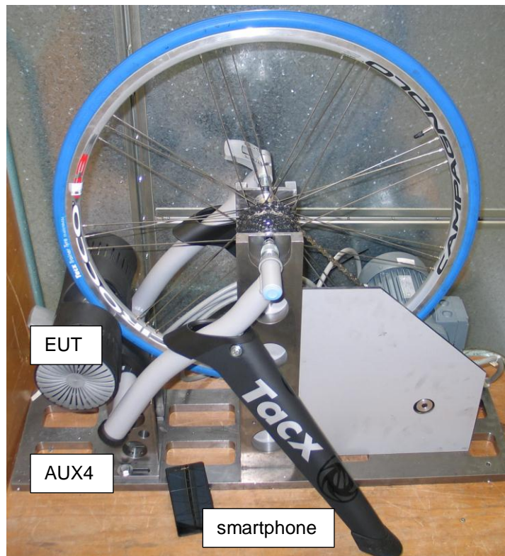
Figure 2. Basic set-up for testing
