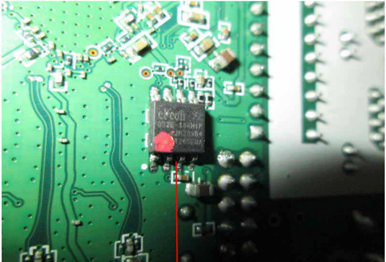
SPI flash for Wifi SOC
