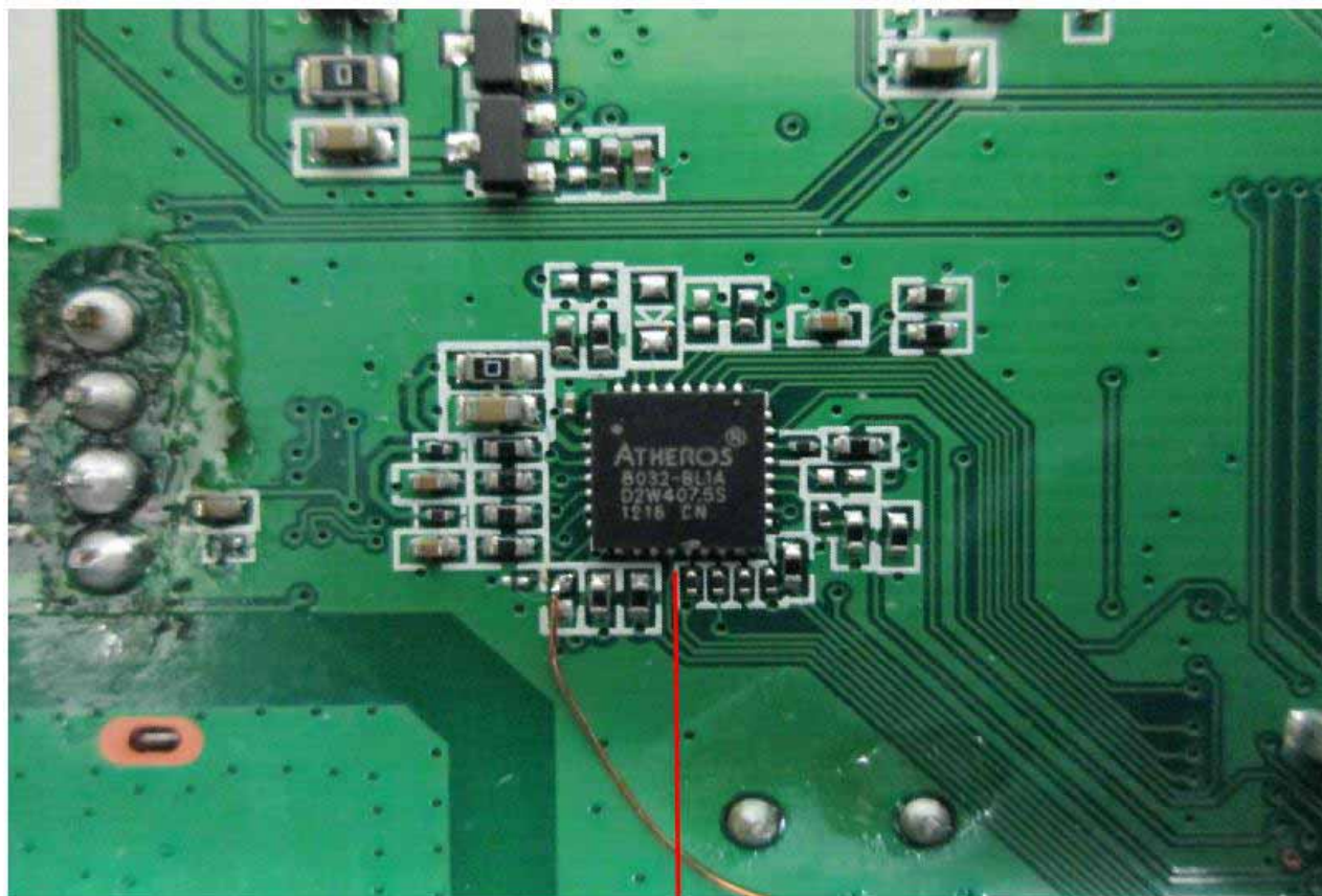
Ethernet phy
