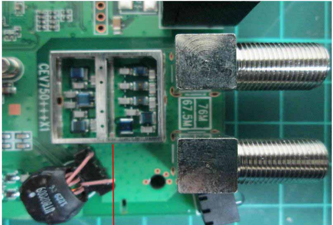
Diplexer
