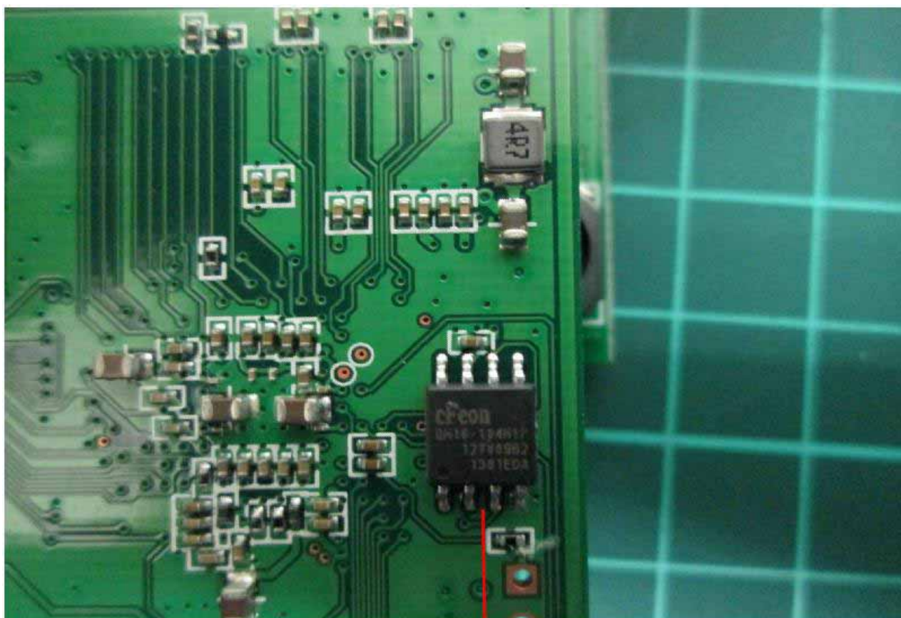
SPI flash for PLC Transceiver
