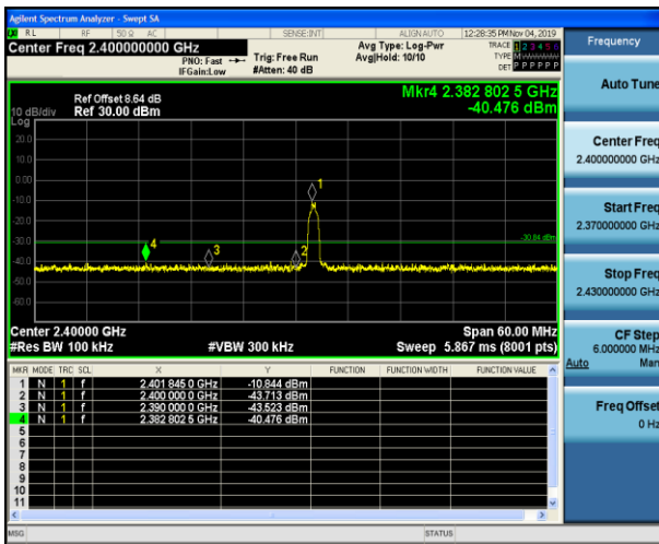
No-hopping mode
