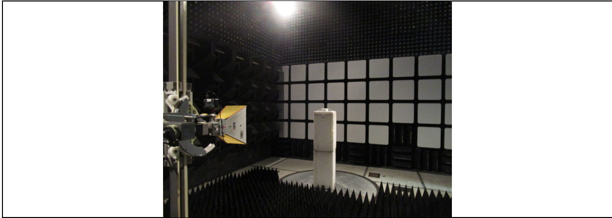
Radiated Emissions
