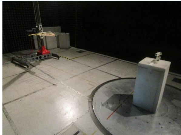
Radiated Emission Below 1 GHz Setup
