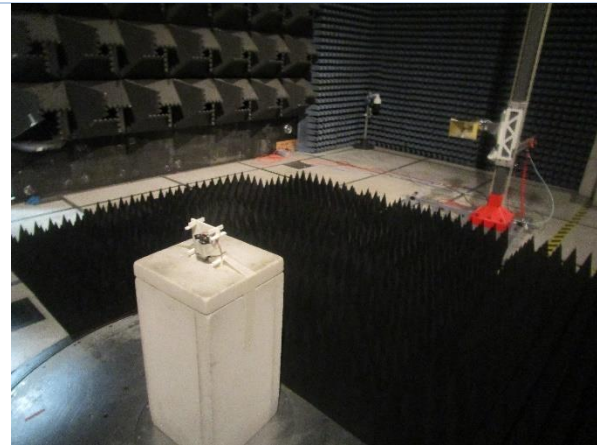
Radiated Emissions Above 1 GHz Setup
