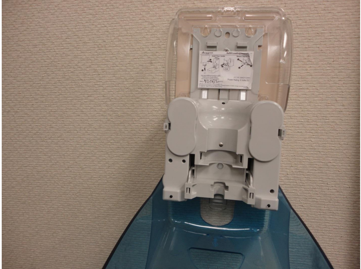
Figure 11: Close-up of FCC Label Mounted on Dispenser (SKU 52062)
