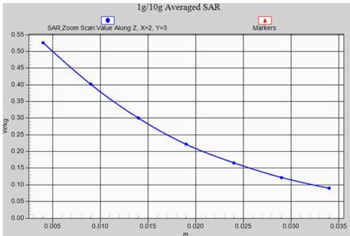
GSM850 Back side-High with headset_ z-axis scan
