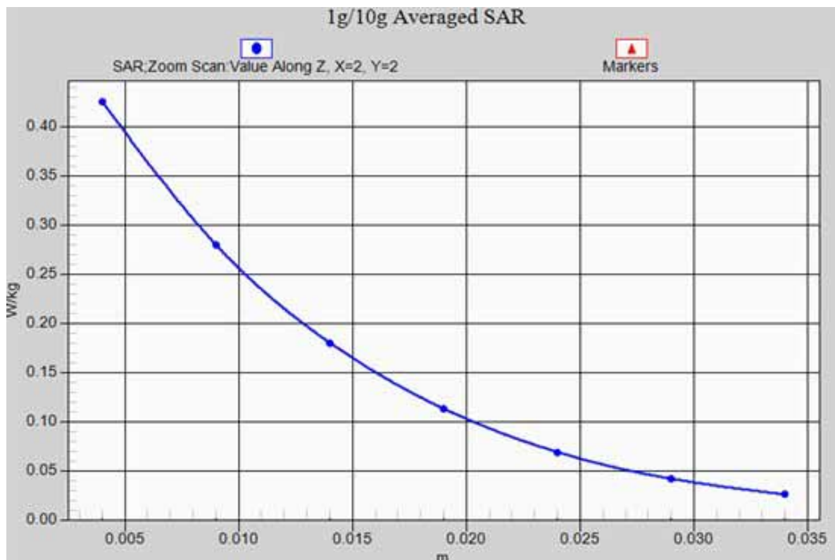
PCS1900 RIGHT/CHEEK-Mid_ z-axis scan
