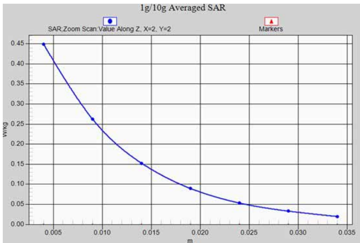
GSM1900 Back side-Mid with headset_ z-axis scan
