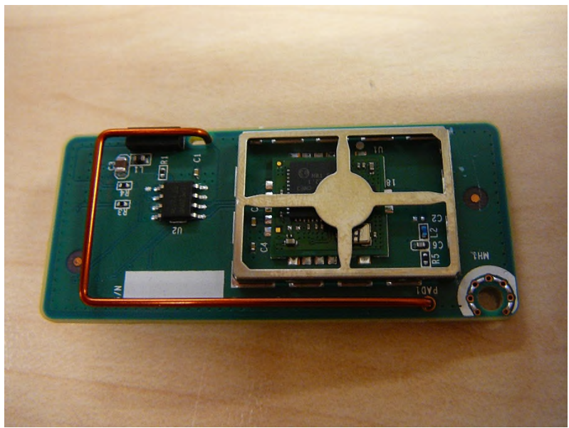
QS-ZwaveAH – Top View with Cover Removed
