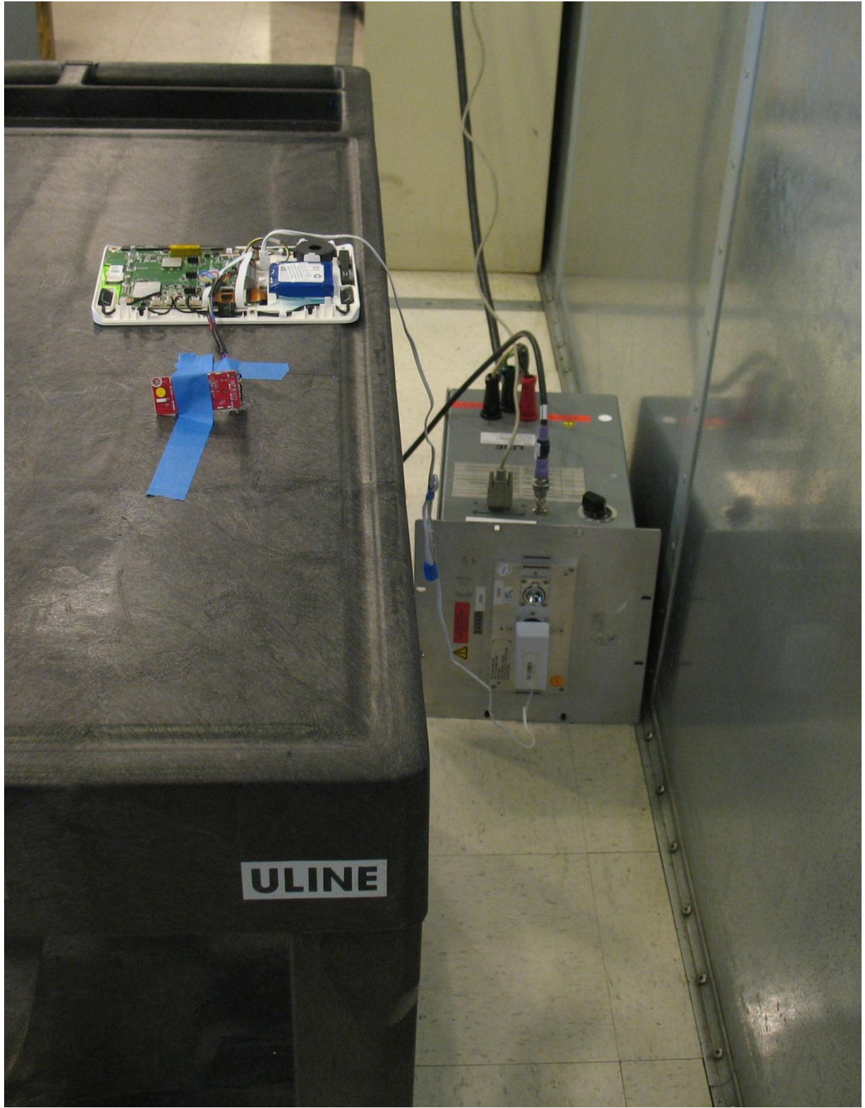
Conducted Emissions
