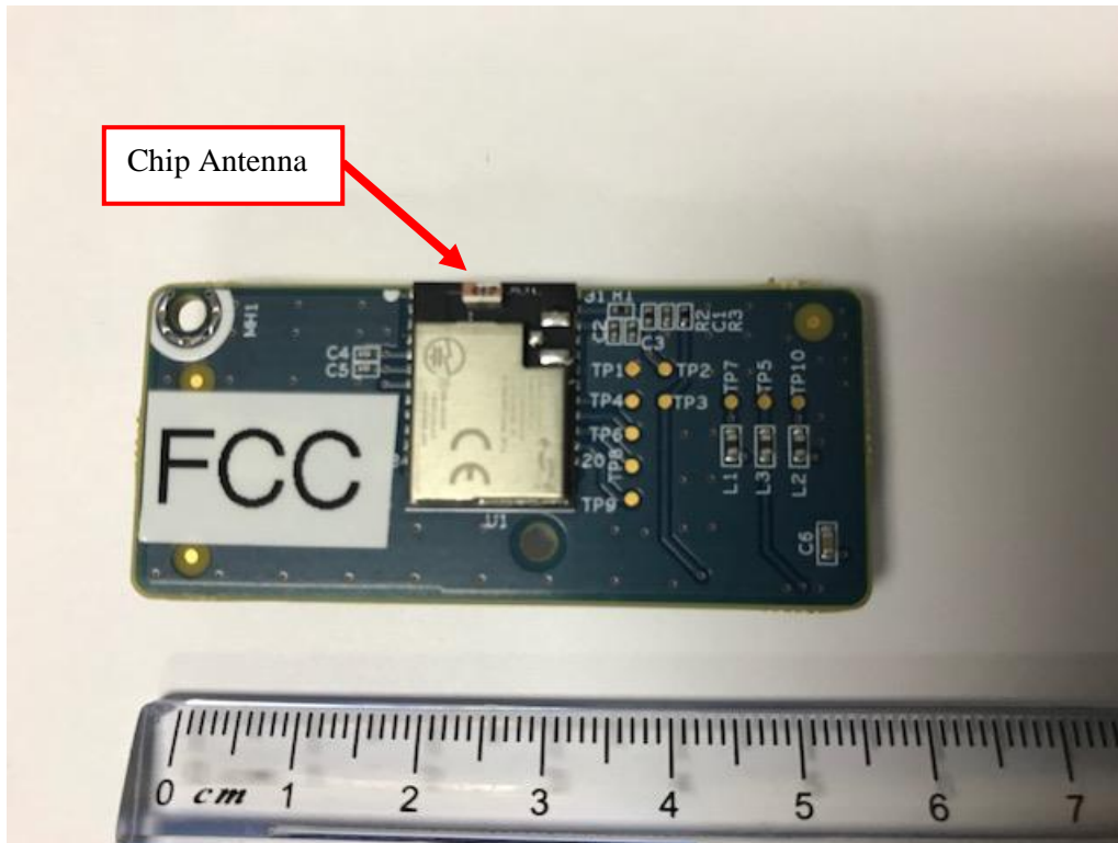
Figure 1: External Picture Qolsys Zigbee Radio Card - QS-ZB – Radiated Sample - Top
