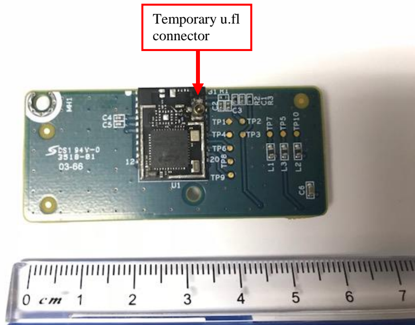
Figure 3: External Picture Qolsys Zigbee Radio Card - QS-ZB – Conducted test sample - Top
