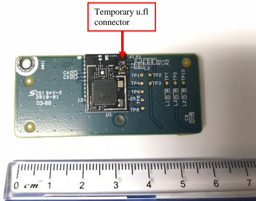
Figure 3: Internal Picture Qolsys Zigbee Radio Card - QS-ZB – Conducted test sample - Top
