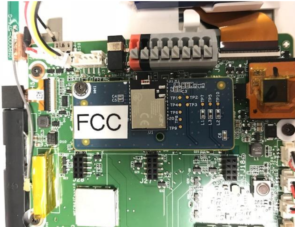
Figure 6: Picture Qolsys Zigbee Radio Card – Radiated Test Sample - Connected to auxiliary host QS-IQPANEL2 card slot – Informative only
