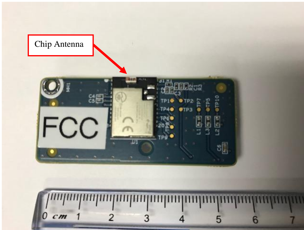
Figure 1: Internal Picture Qolsys Zigbee Radio Card - QS-ZB – Radiated Sample - Top
