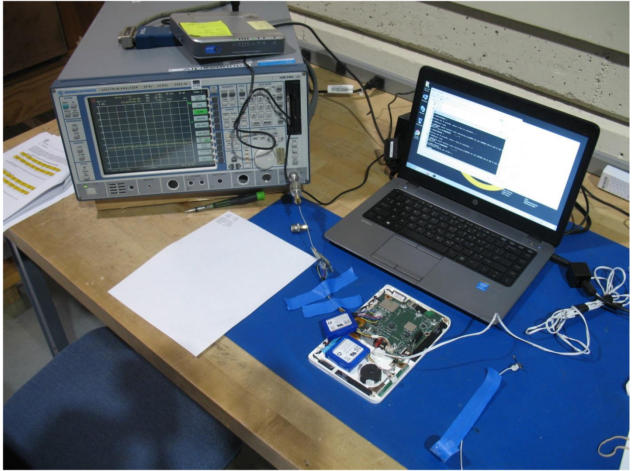
Benchtop Measurements
