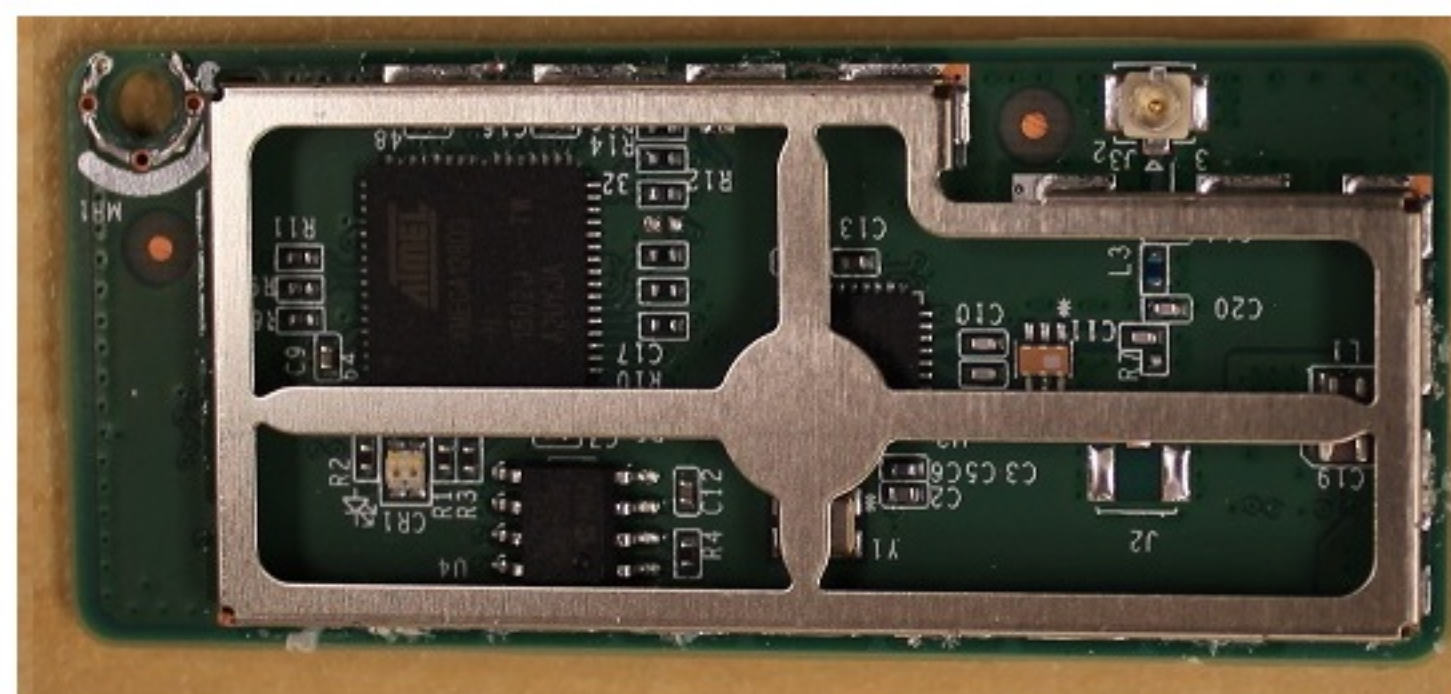
Top View, Shield top removed
