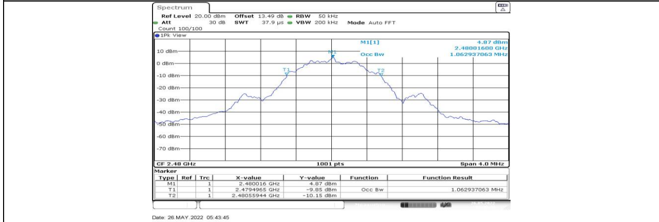
BLE_1M_Ant1_2480
