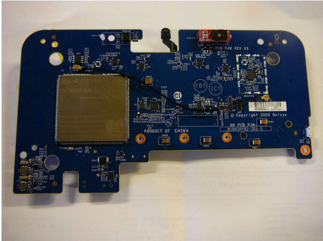
Main PCBA – Top Side
