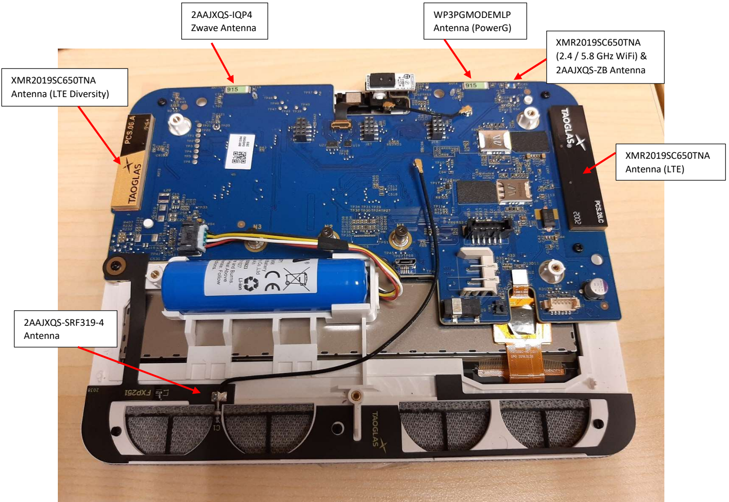
Main PCB with no optional Cards installed – Bottom Side
