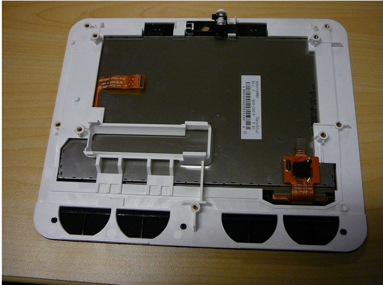
Front of Panel showing LCD
