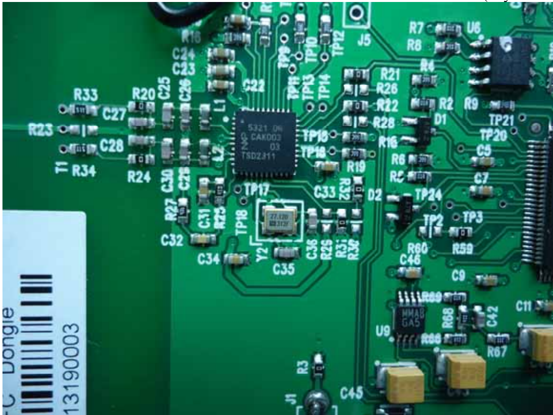
Figure 9 Main Board (Crystal Oscillator)
