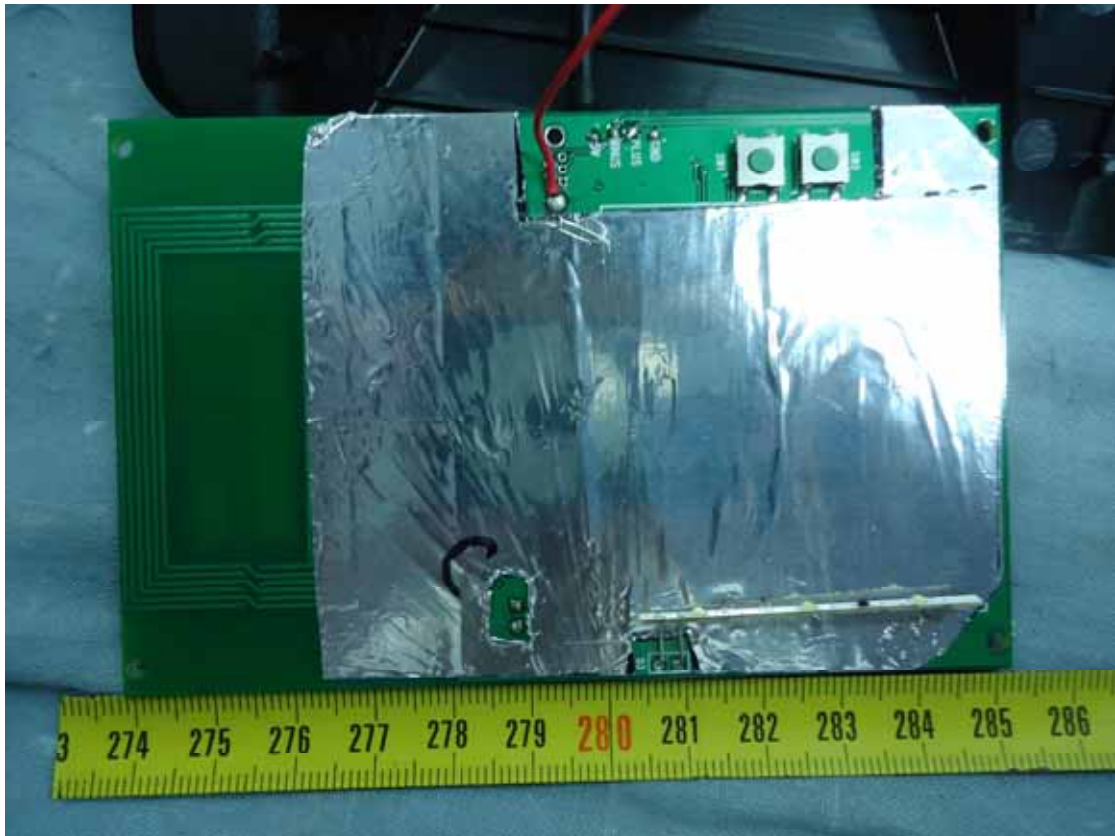
Figure 5 Aluminum Foil
