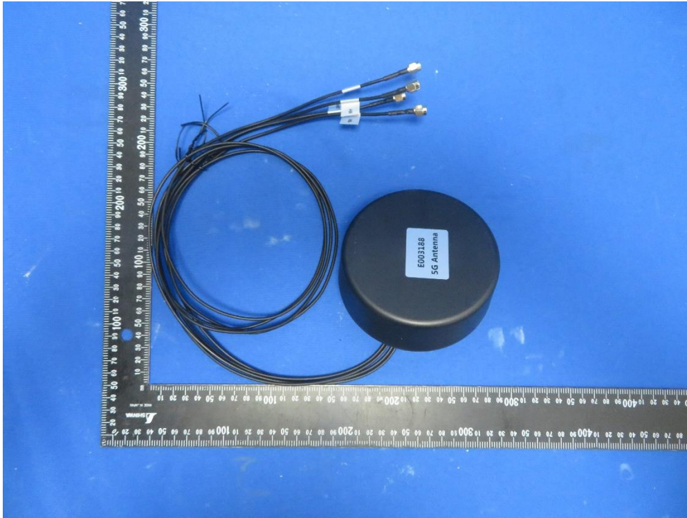
(11) EUT Photo – GNSS/WWAN Antenna #1
